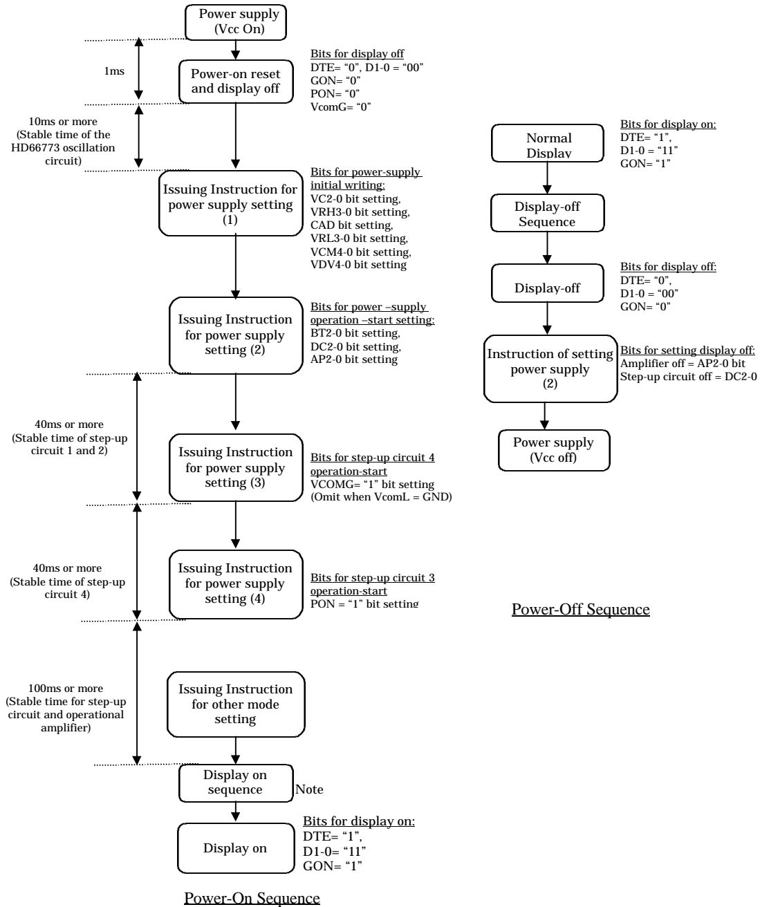
Figure 97 Flow of Power-Supply Setting
