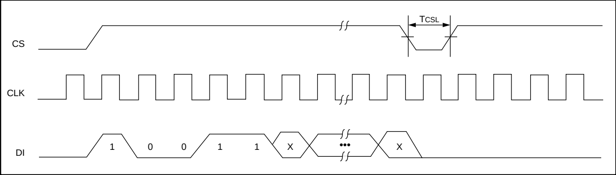
FIGURE 3-5: EWEN TIMING
