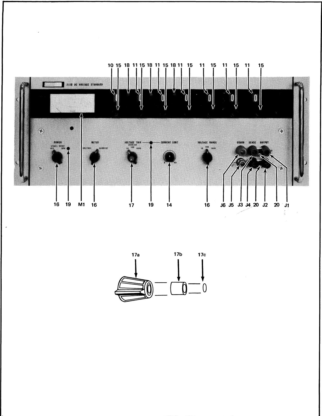
Figure 5-1. DC VOLTAGE STANDARD (Sheet 3 of 3)
