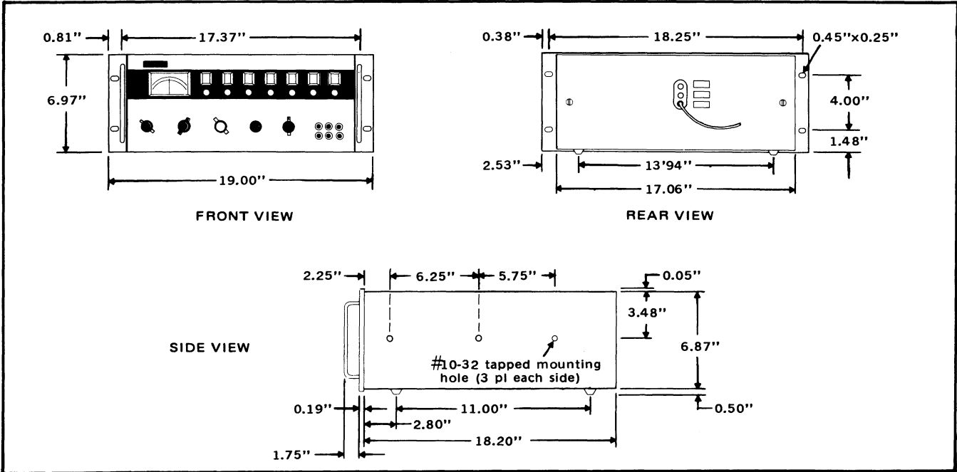
Figure 1-1. MODEL 332D OUTLINE DRAWING
