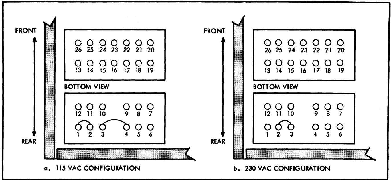
Figure 4-1. 115/230 VAC CONVERSION
