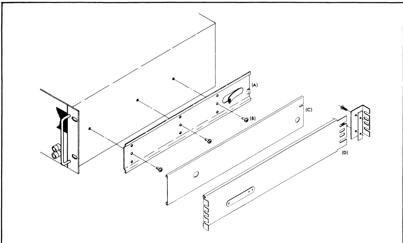
Figure 2-1. CHASSIS SLIDE INSTALLATION
