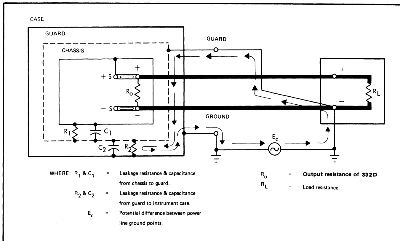
Figure 2-4. GUARD CONNECTION
