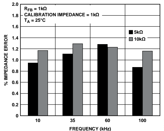
Figure 27. Impedance Range 2 Typical % Impedance Error over Frequency
