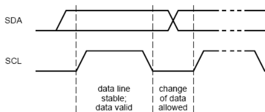
Figure 6-1. IIC data to clock protocol
