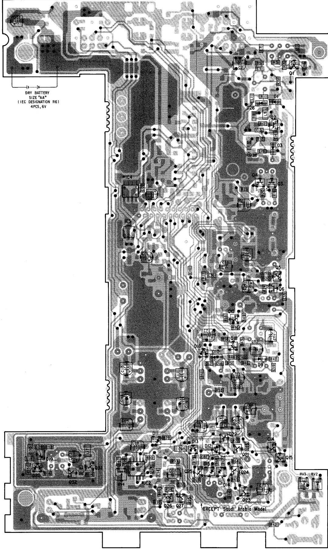
[MAIN BOARD] (SIDE B)
