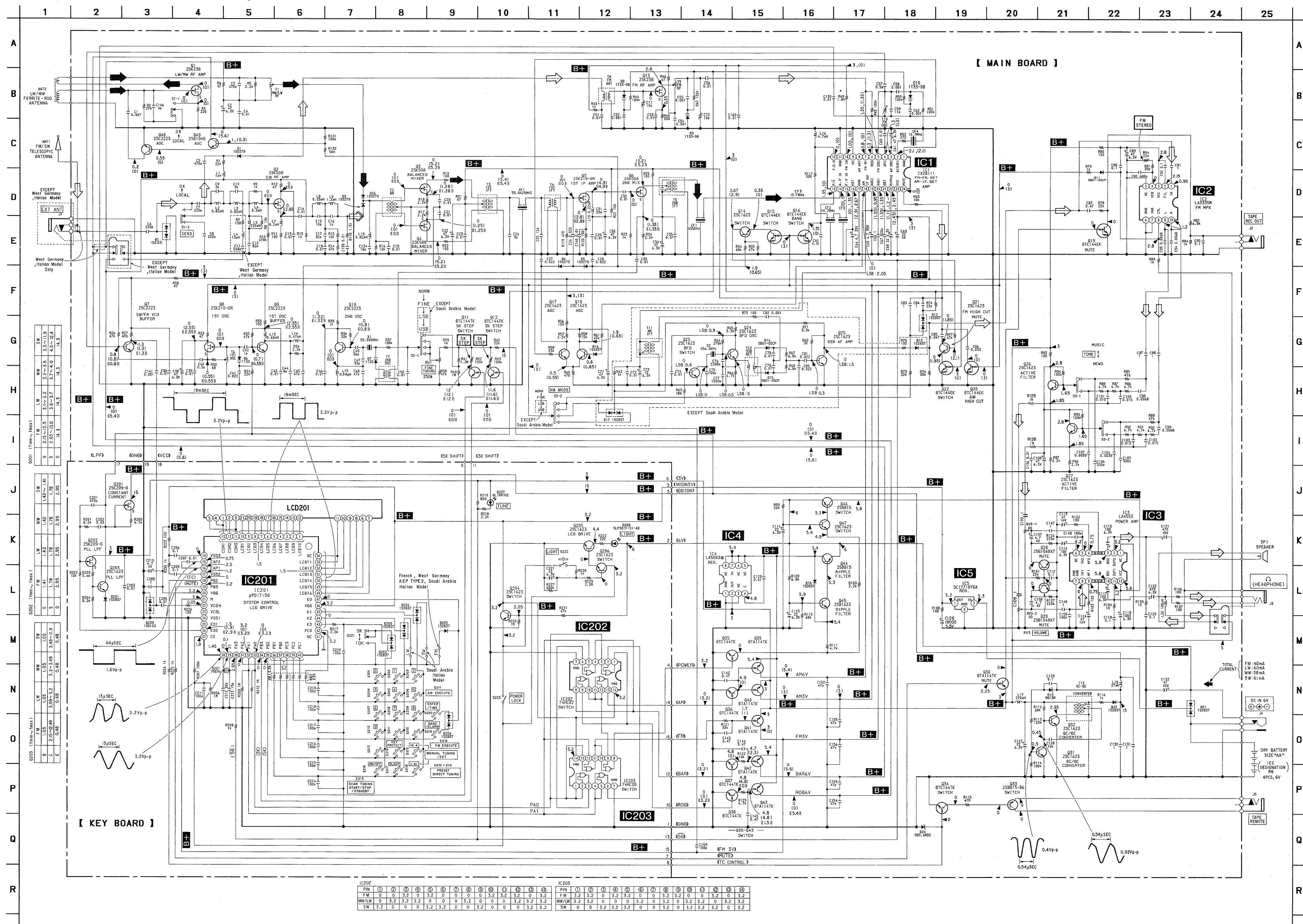
5-3. SCHEMATIC DIAGRAM • See page 17 for IC Block Diagrams.
