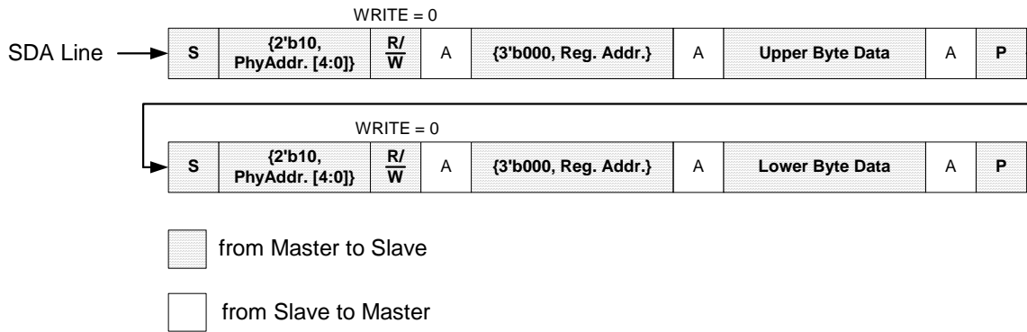
Figure 23: Random Write Operation
