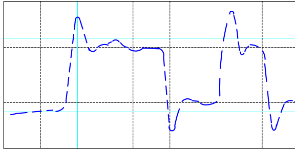
Figure 34: Signal Reflections, using the 50 ohm Setting, 60 ohm line
