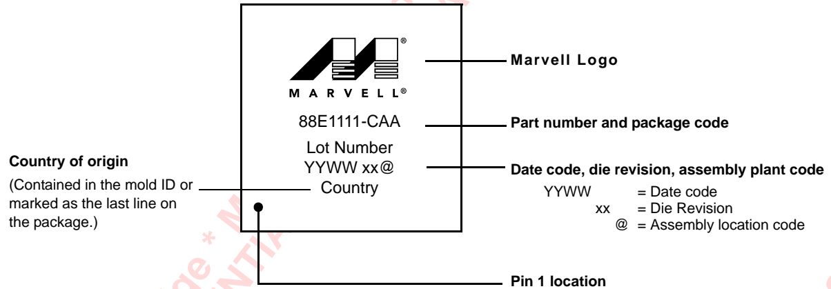
Figure 80: 88E1111 96-pin BCC Commercial Package Marking and Pin 1 Location
