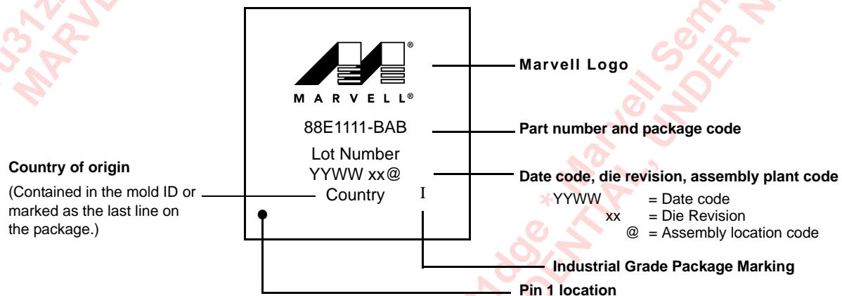
Figure 79: 88E1111 117-pin TFBGA Industrial Package Marking and Pin 1 Location
