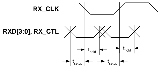
Figure 56: RGMII RX_CLK Delay Timing - Register 20.7 = 1 (add delay)
