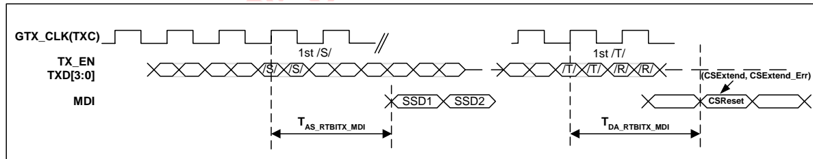
Figure 68: RTBI to 1000BASE-T Transmit Latency Timing
