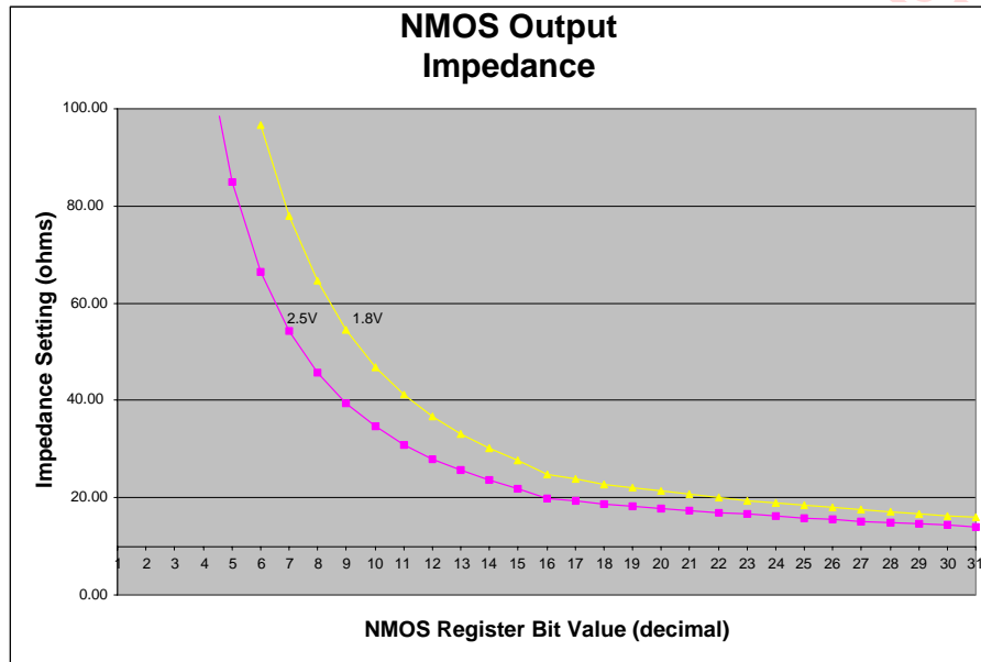
Figure 33: NMOS Output Impedance (1.8V, 2.5V) Trend Lines
