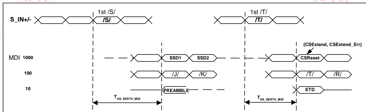
Figure 70: SGMII to 10/100/1000BASE-T Transmit Latency Timing
