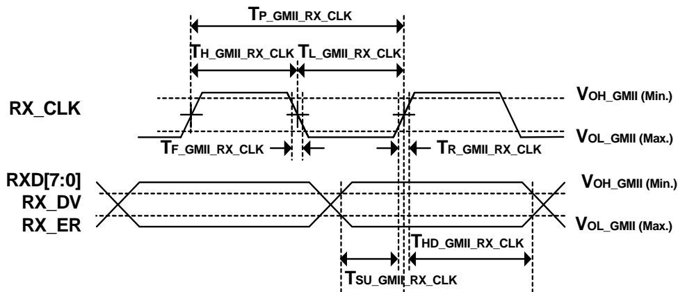
Figure 47: GMII Receive Timing
