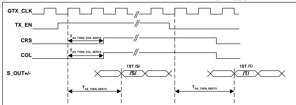
Figure 60: GMII to 1000BASE-X Transmit Latency Timing
