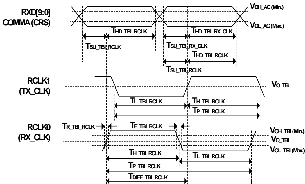
Figure 51: TBI Receive Timing
