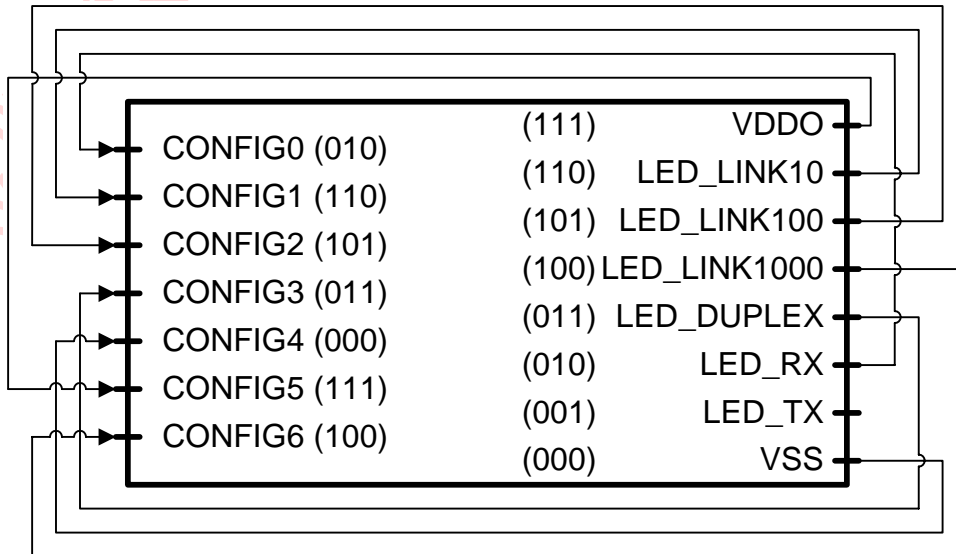
Figure 19: Configuration Connection Example
