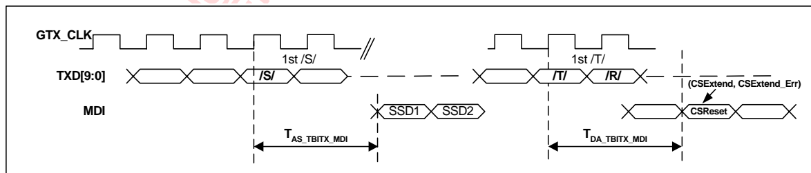
Figure 66: TBI to 100BASE-T Transmit Latency Timing
