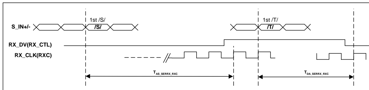
Figure 65: 1000BASE-X to RGMII Receive Latency Timing
