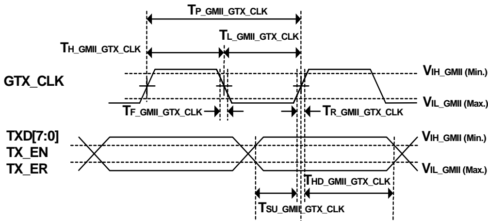
Figure 46: GMII Transmit Timing
