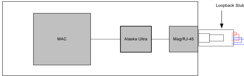
Figure 31: Test Setup for 10/100/1000 Mbps Modes using an External Loopback Stub
