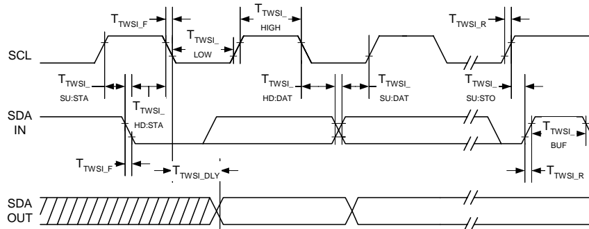
Figure 75: Two-Wire Serial Interface Timing
