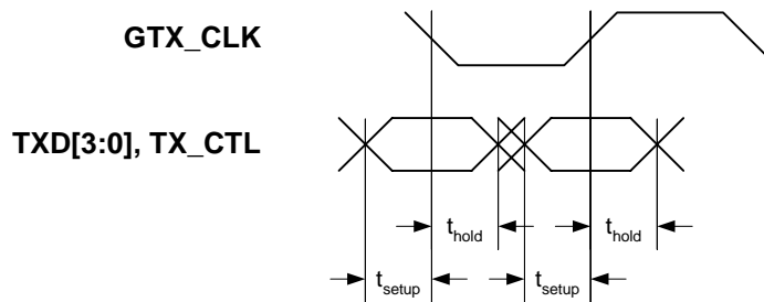
Figure 53: GTX_CLK Delay Timing - Register 20.1 = 0
