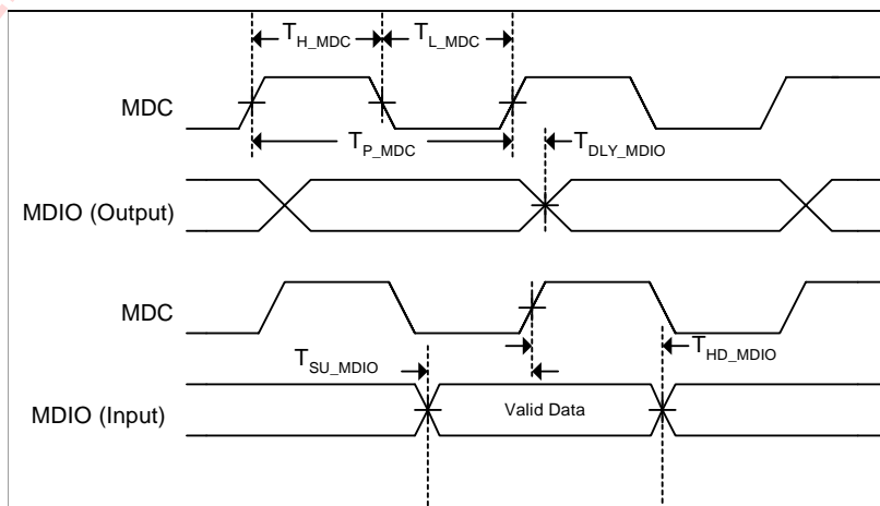
Figure 74: Serial Management Interface Timing
