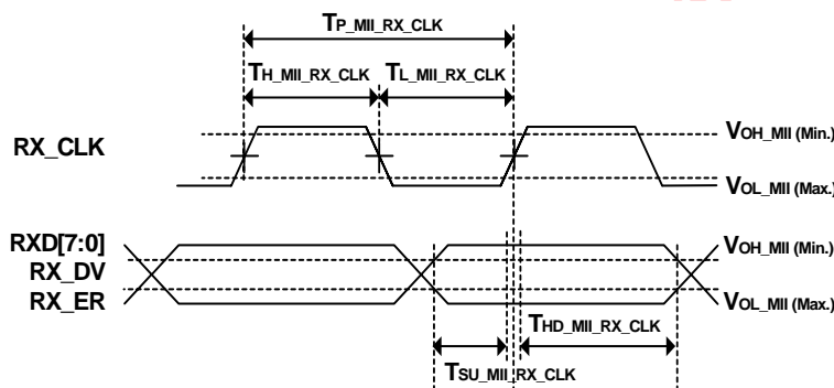
Figure 49: 10/100 Mbps Receive Timing
