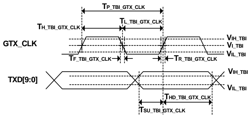
Figure 50: TBI Transmit Timing
