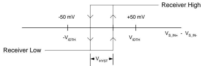
Figure 42: Input Differential Hysteresis
