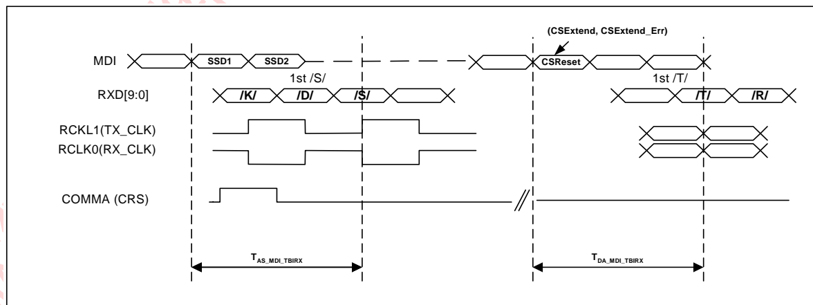
Figure 67: 1000BASE-T to TBI Receive Latency Timing
