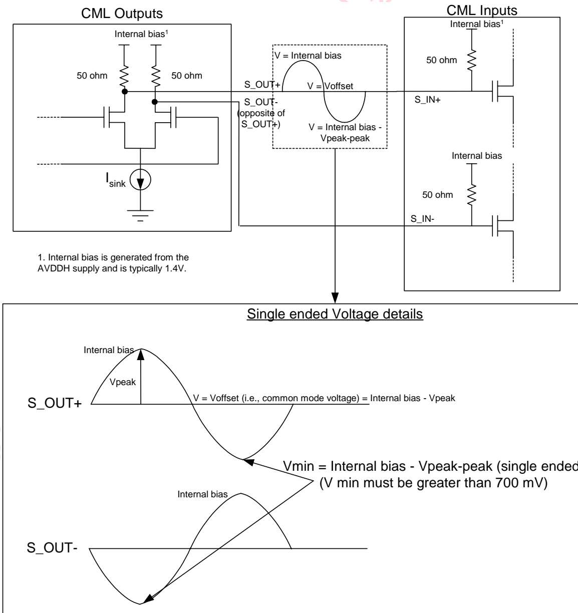
Figure 41: DC connection to a CML receiver
