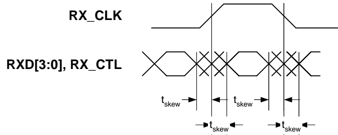
Figure 55: RGMII RX_CLK Delay Timing - Register 20.7 = 0
