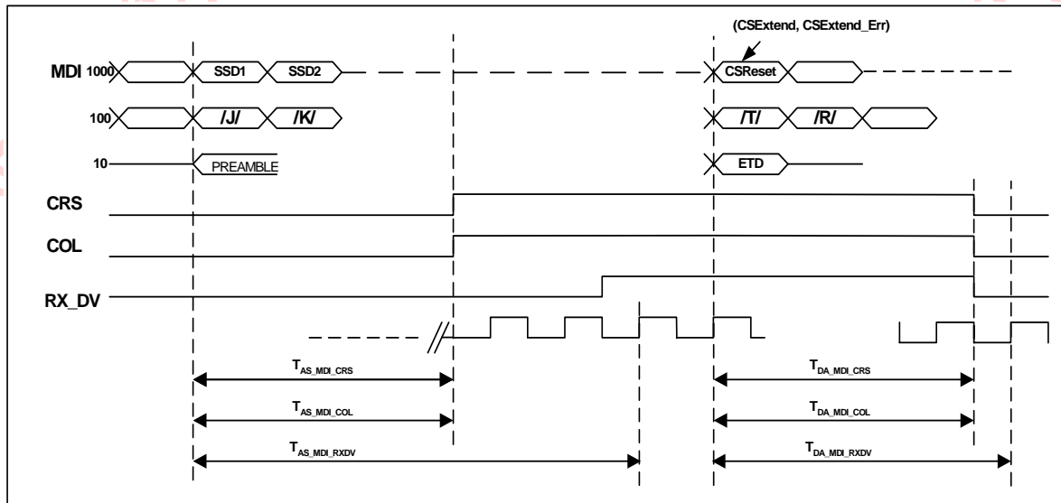
Figure 59: 10/100/1000BASE-T to GMII/MII Receive Latency Timing
