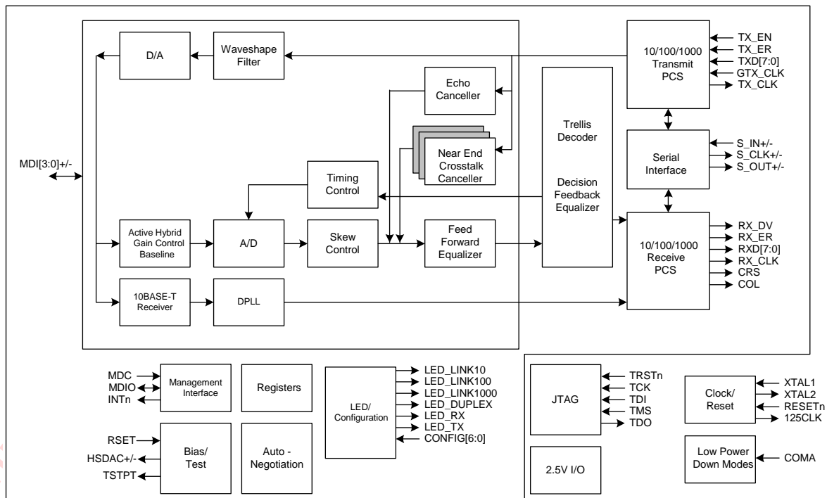
Figure 5 shows the functional block diagram of the 88E1111 device. The transmitter and transmit PCS and PMA blocks are more fully described on “Transmit Side Network Interface” on page 70. The receiver and receive PCS and PMA blocks are more fully described on “Receive Side Network Interface” on page 70.
