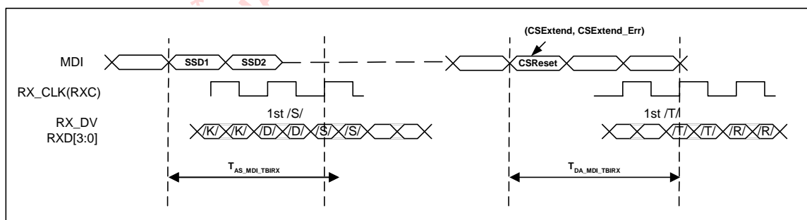
Figure 69: 1000BASE-T to RTBI Receive Latency Timing
