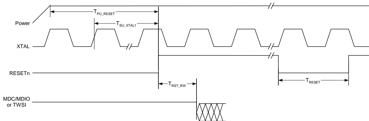
Figure 43: Reset Timing
