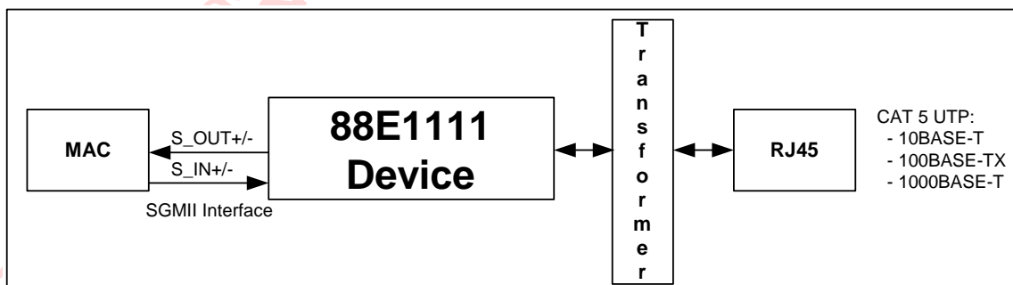
Figure 16: SGMII Interface
