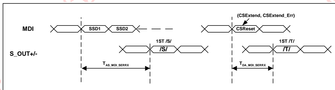
Figure 73: 1000BASE-T to 1000BASE-X Receive Latency Timing
