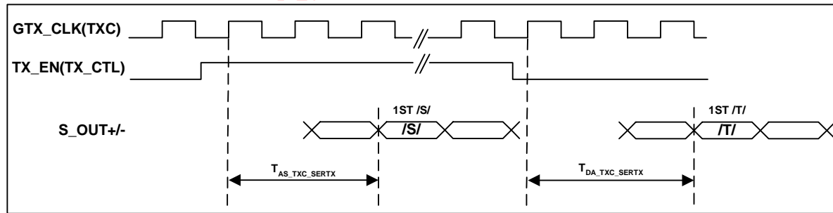
Figure 64: RGMII to 1000BASE-X Transmit Latency Timing
