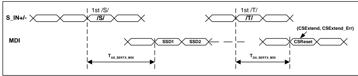
Figure 72: 1000BASE-X to 1000BASE-T Transmit Latency Timing
