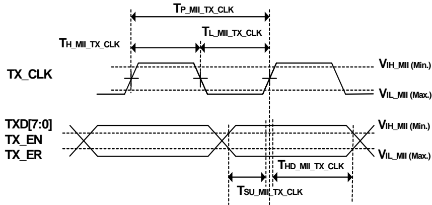
Figure 48: 10/100 Mbps Transmit Timing
