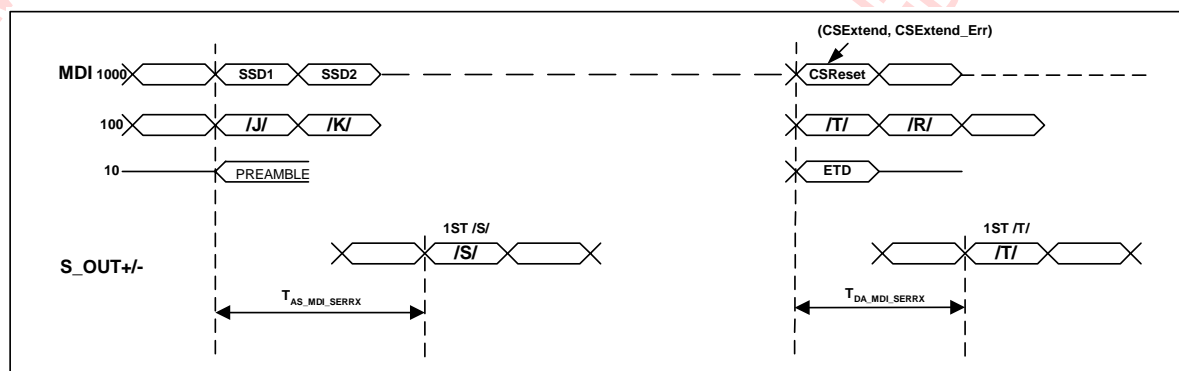
Figure 71: 10/100/1000BASE-T to SGMII Receive Latency Timing
