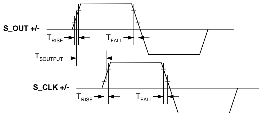
Figure 57: Serial Interface Rise and Fall Times
