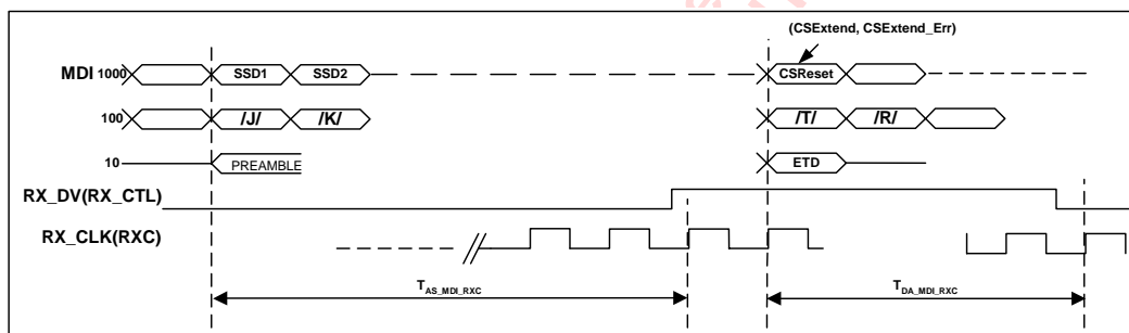
Figure 63: 10/100/1000BASE-T to RGMII Receive Latency Timing
