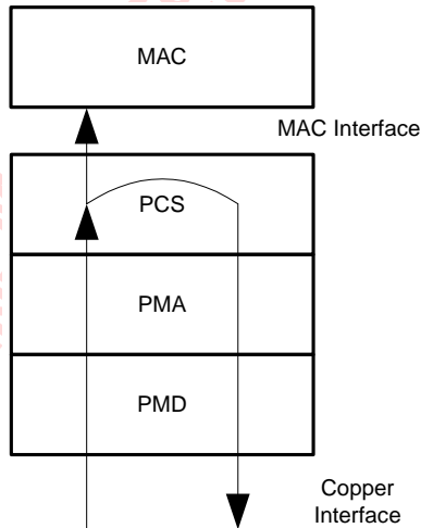
Figure 29: Line Loopback Data Path
