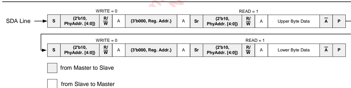
Figure 26: Random Read Operation
