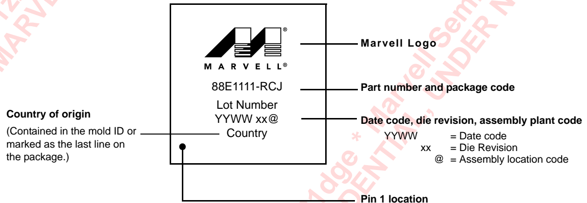
Figure 81: 88E1111 128-pin PQFP Commercial Package Marking and Pin 1 Location
