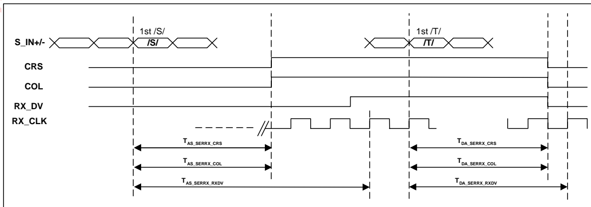
Figure 61: 1000BASE-X to GMII Receive Latency Timing
