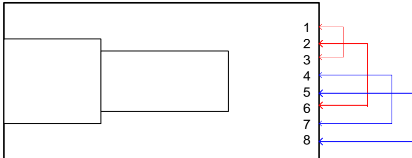
Figure 30: Loopback Stub (Top View with Tab up)
