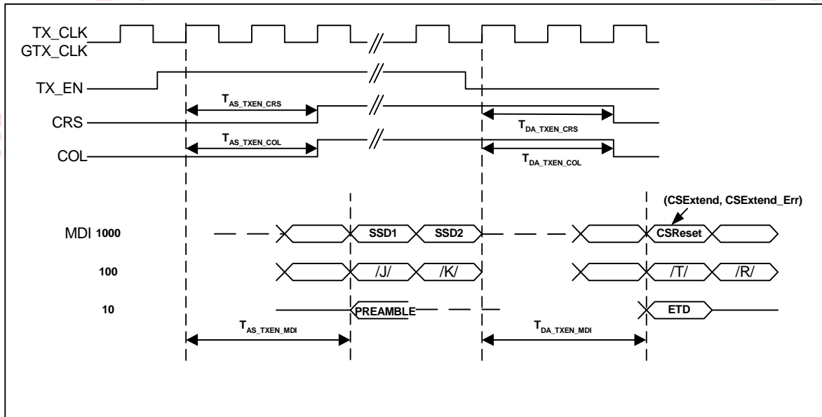
Figure 58: GMII/MII to 10/100/1000BASE-T Transmit Latency Timing
