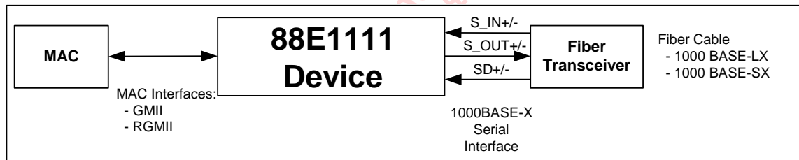
Figure 18: MAC to Fiber Connection
