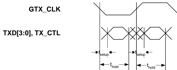
Figure 54: GTX_CLK Delay Timing - Register 20.1 = 1 (add delay)
