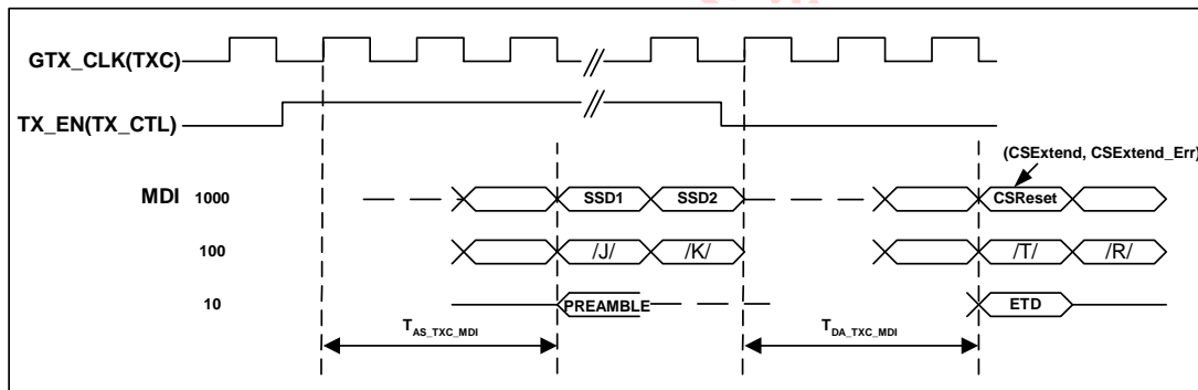
Figure 62: RGMII/MII to 10/100/1000BASE-T Transmit Latency Timing
