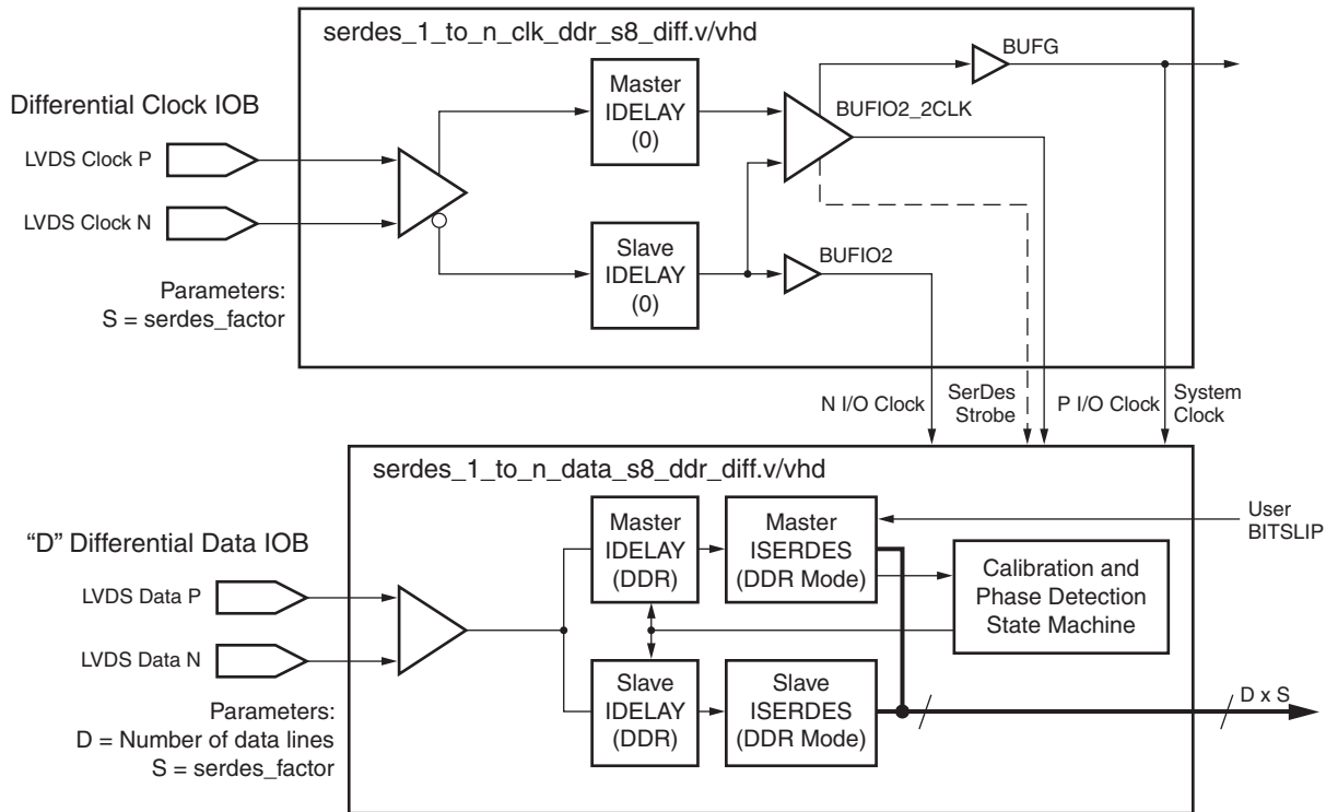
Figure 6: DDR Data Reception Using Two BUFIO2s
