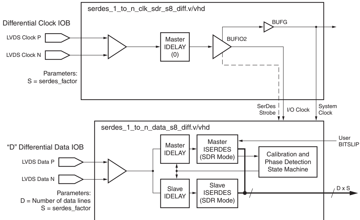
Figure 7: SDR Data Reception Using BUFIO2
