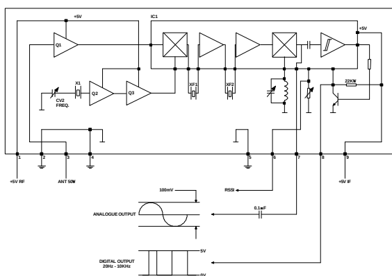
Figure 3: Narrow Band Transmitter and Receiver Block Diagrams
