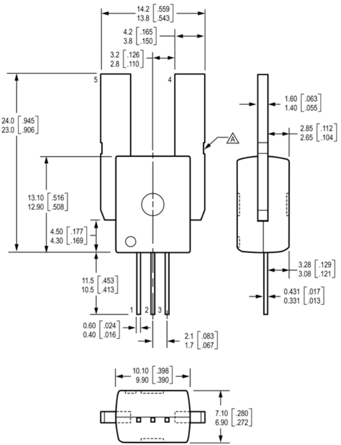
Package CB-PSS
