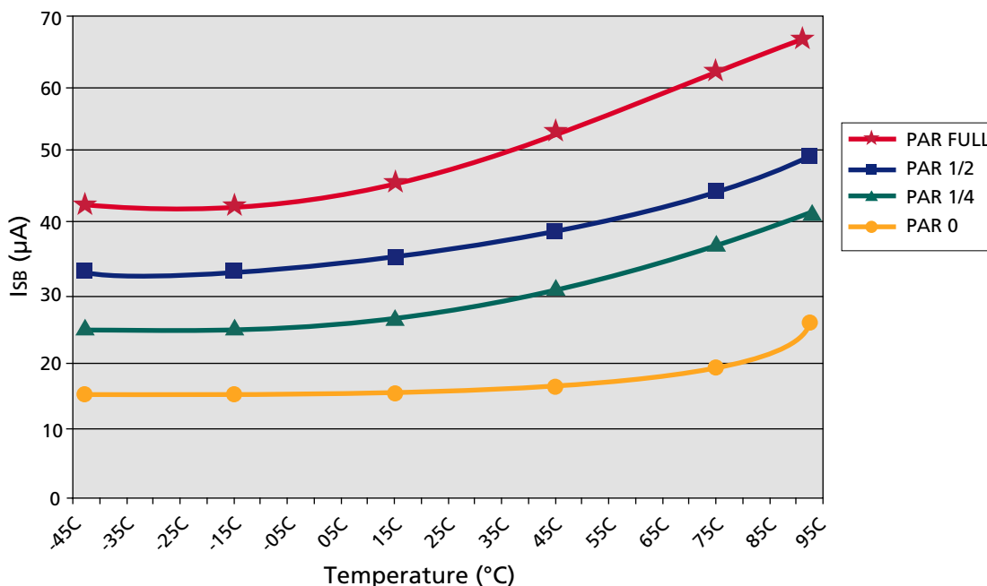
Figure 13: Typical Refresh Current vs. Temperature
