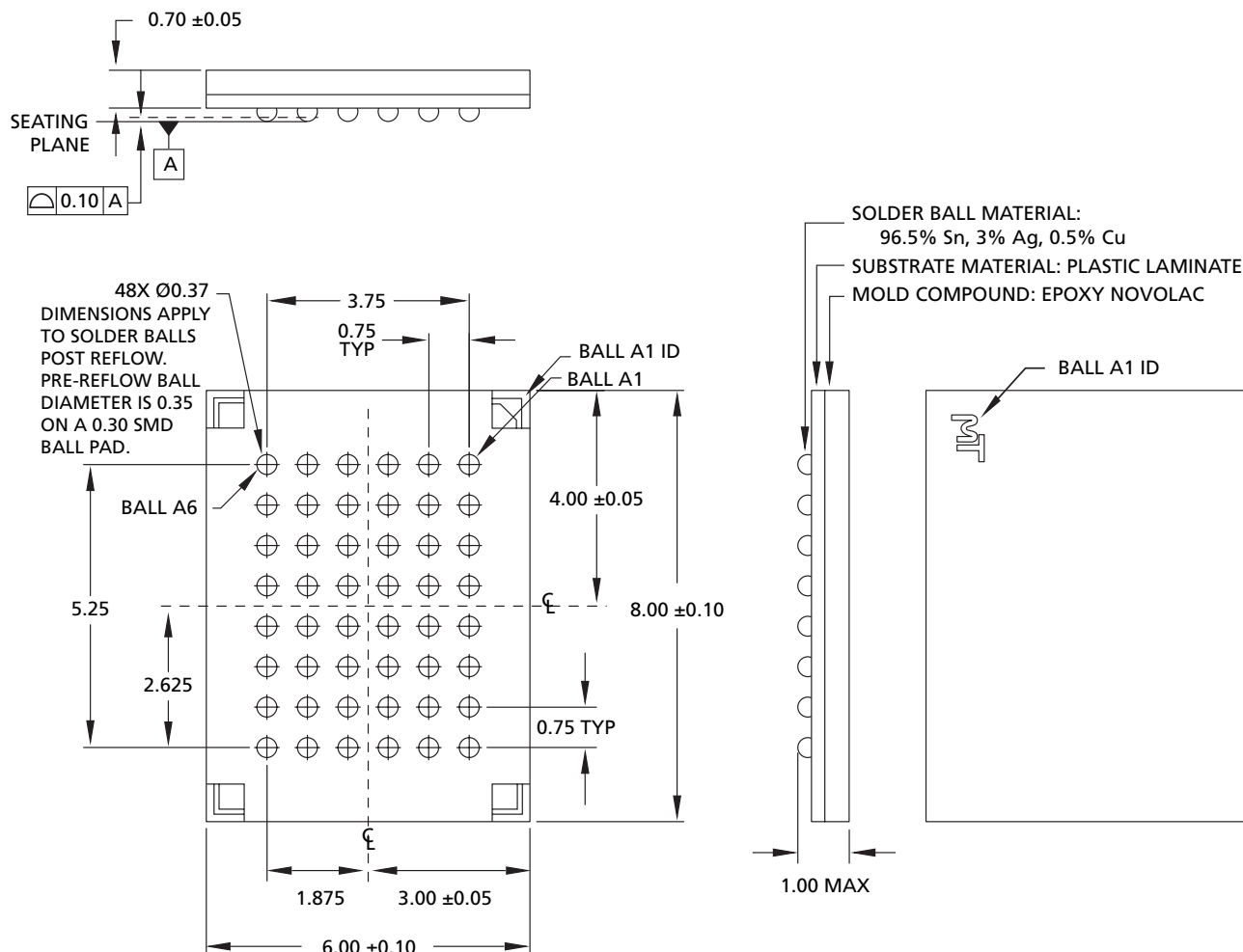
Figure 24: 48-Ball VFBGA
