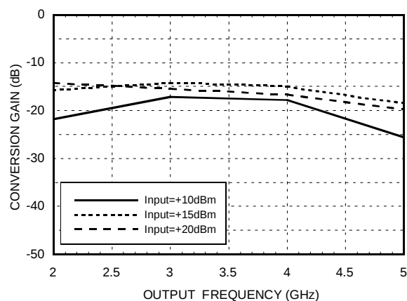
Conversion Loss vs. Drive Level
