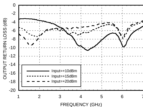
Output Return Loss vs. Drive Level
