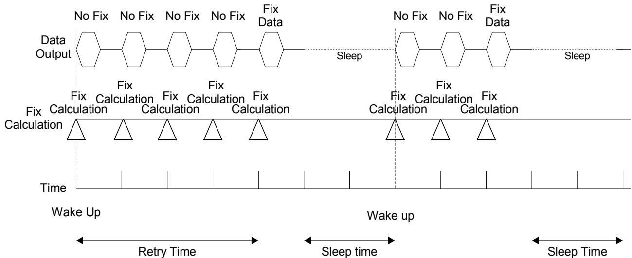
Fig-2. Recovery From Sleep to Position Calculation
