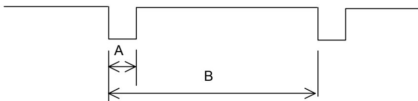
Fig-5. Wake Up Signal
