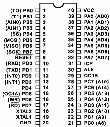
Abb. 3: Pin-Configuration des AT90S8515 (PDIP-Gehäuse)
