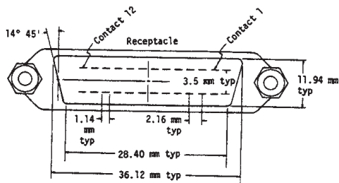
Figure 17—Receptacle Dimensions
