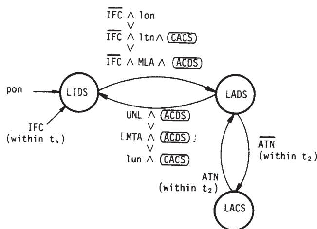
Figure 7—L State Diagram
