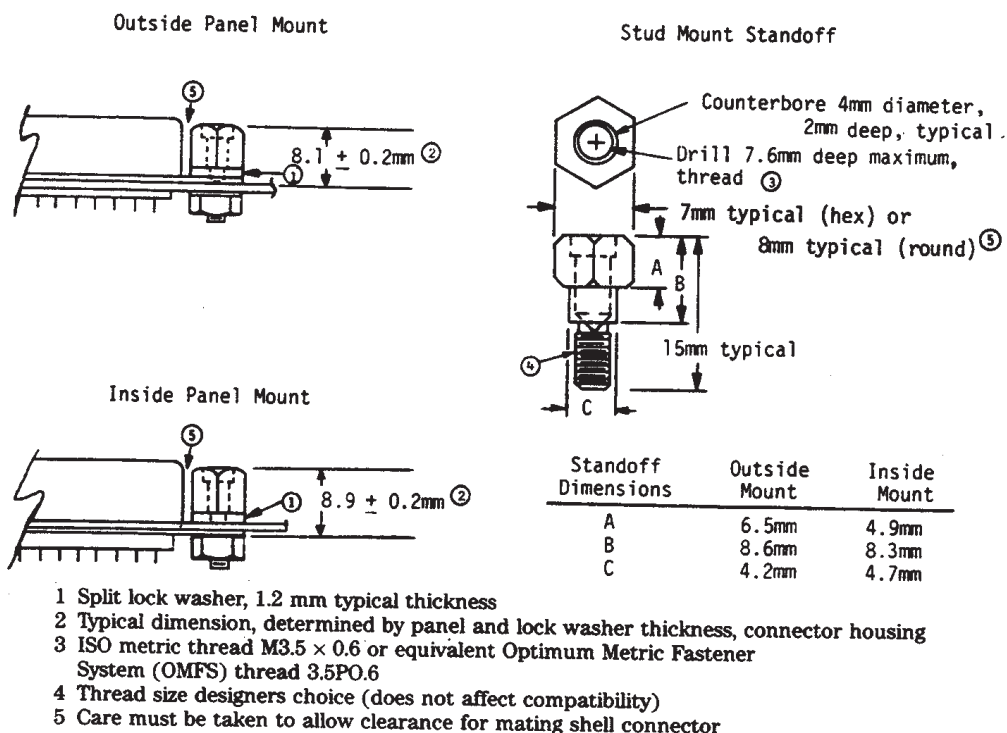
Figure 19—Mounting Dimensions
