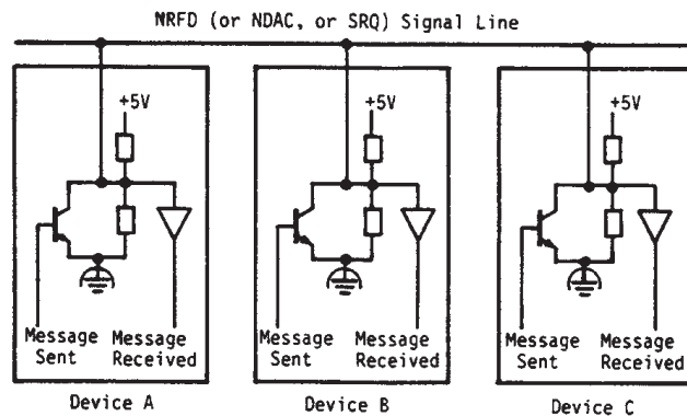
Figure 23—Bi-State Signal Line Logic (Open Collector Drivers)
