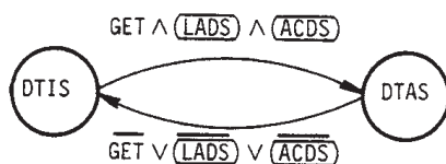
Figure 13—DT State Diagram
