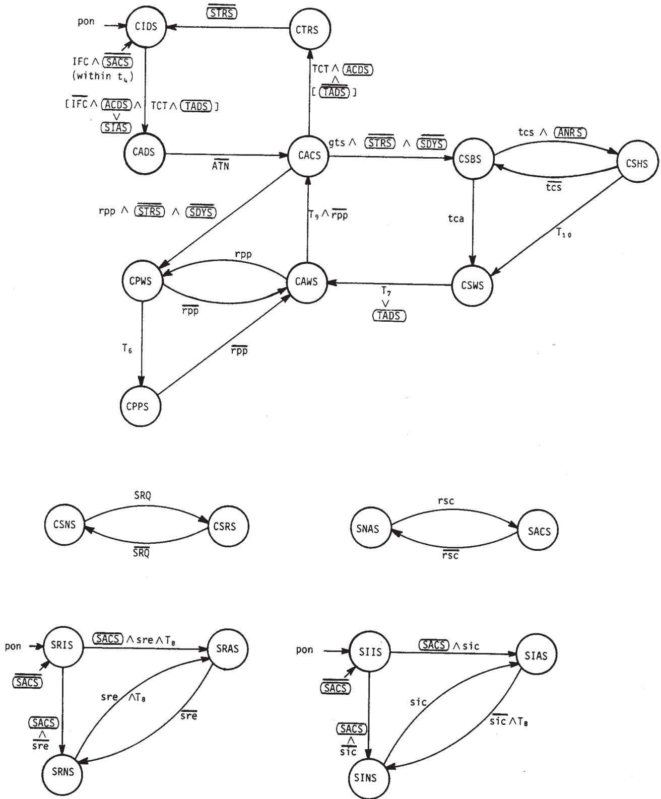
Figure 14—C State Diagram
