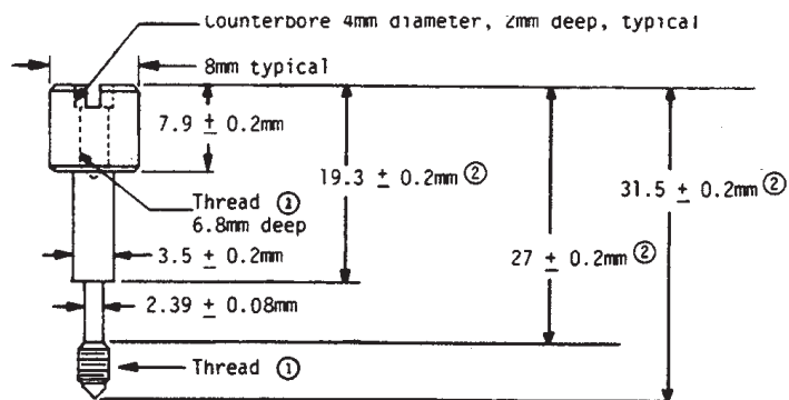
1 = ISO metric thread M3.5×0.6 or equivalent O.M.F.S. thread 3.5PO.6 2 Length is function of housing dimension
