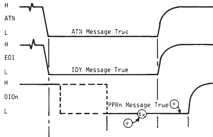
Figure G.1—Parallel Poll Sequence: Signal Line Waveforms
