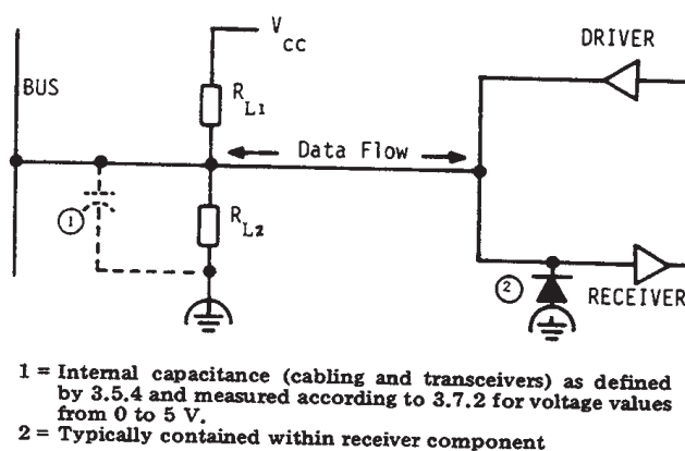
Figure 16—Typical Signal Line Input-Output Circuit
