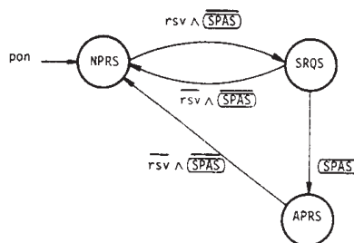
Figure 9—SR State Diagram
