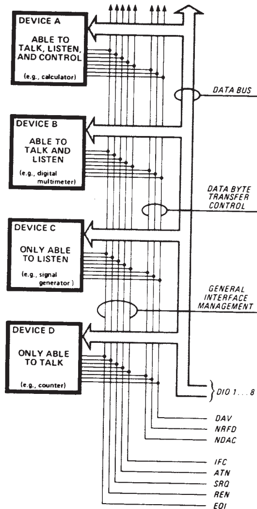
Figure 1—Interface Capabilities and Bus Structure
