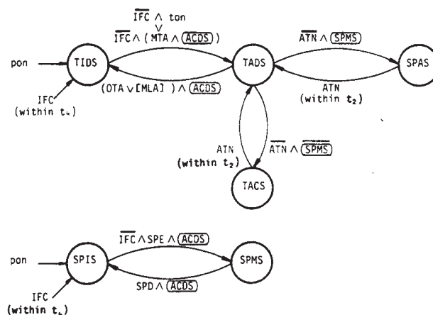
Figure 5—T State Diagram
