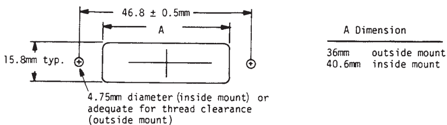
Figure 18—Connector Panel Cutout
