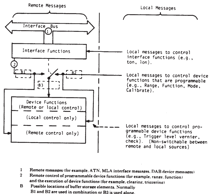
Figure 22—Remote—Local Message Paths
