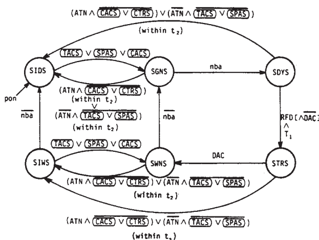
Figure 3—SH State Diagram
