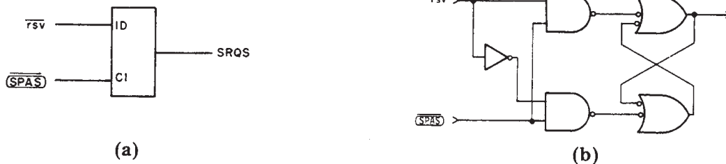
Figure F.1—Partial SR Function — (a) Composite Logic; (b) Gate Level Logic
