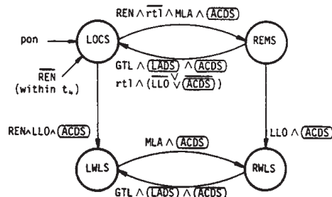
Figure 10—RL State Diagram
