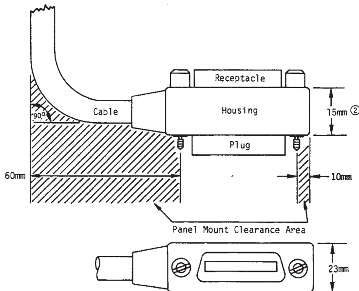
NOTES: (1) All measurements are typical. (2) Length of lock screw is a function of this dimension.
