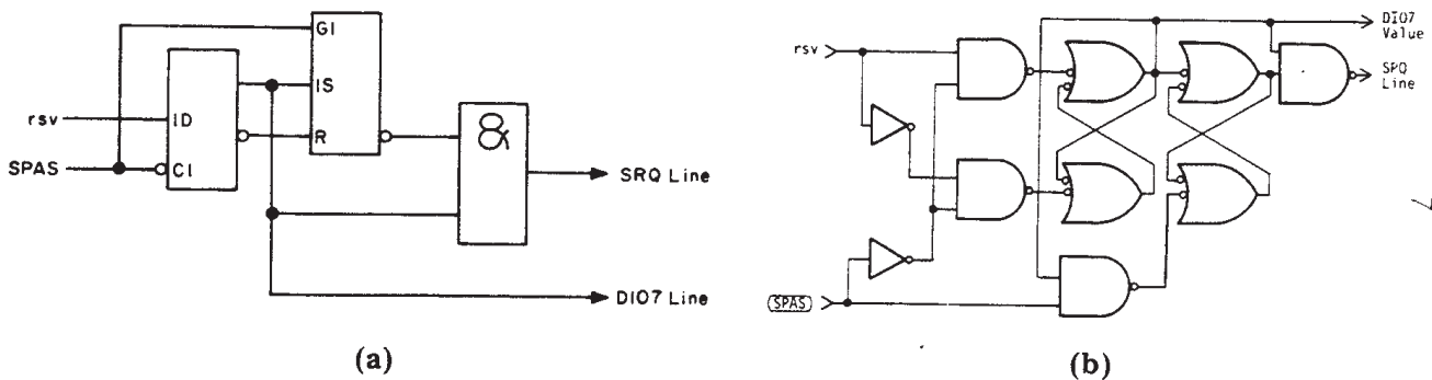
Figure F.2—Full SR Function — (a) Composite Logic; (b) Gate Level Logic
