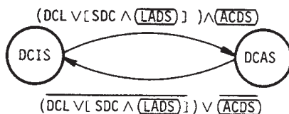
Figure 12—DC State Diagram
