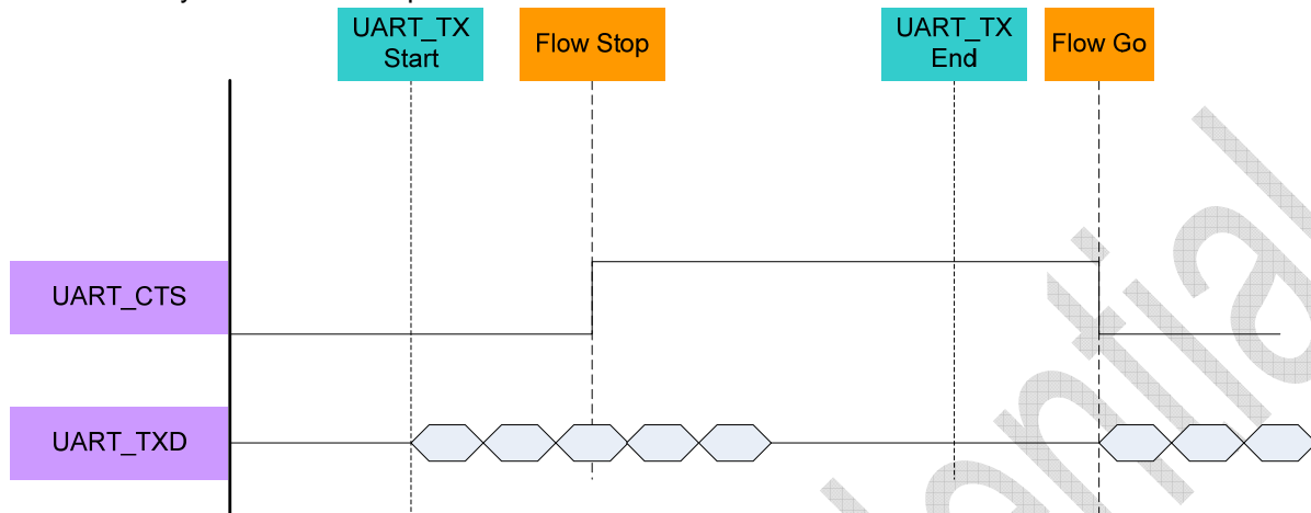
Fig 3.6.1 Host_MCU indicate BM77 UART flow control timing diagram
