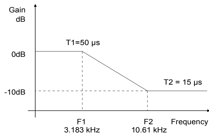
Figure 11. De-Emphasis Curve
