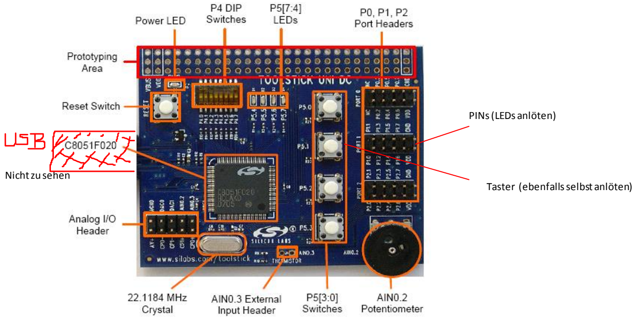
Figure 3. ToolStick University Daughter Card (Rev 002)
