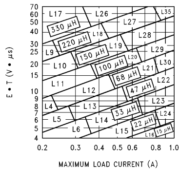
FIGURE 8. LM2595-ADJ
