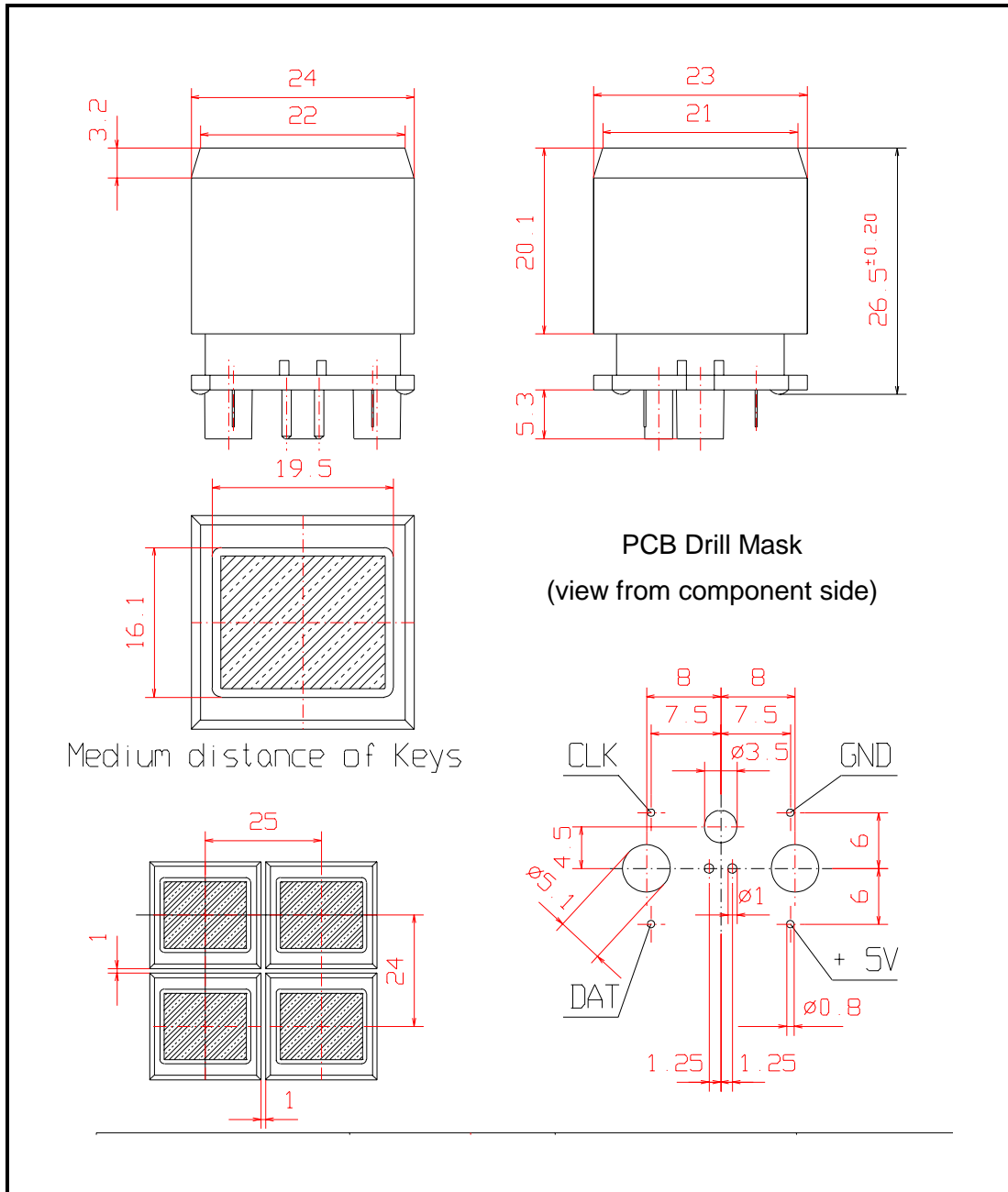
Drawing 2.: Dimensions of LC16.2 Trend ScreenKey in mm. Drill mask view from component side.
