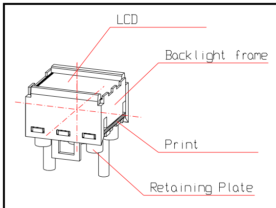
Drawing 3.: LCD Module LC16.2 Trend.
