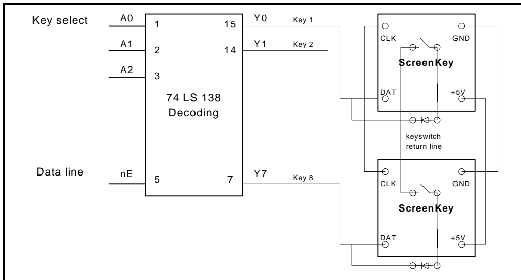
Drawing 7.2.: Decoding circuit LC Trend ScreenKey
