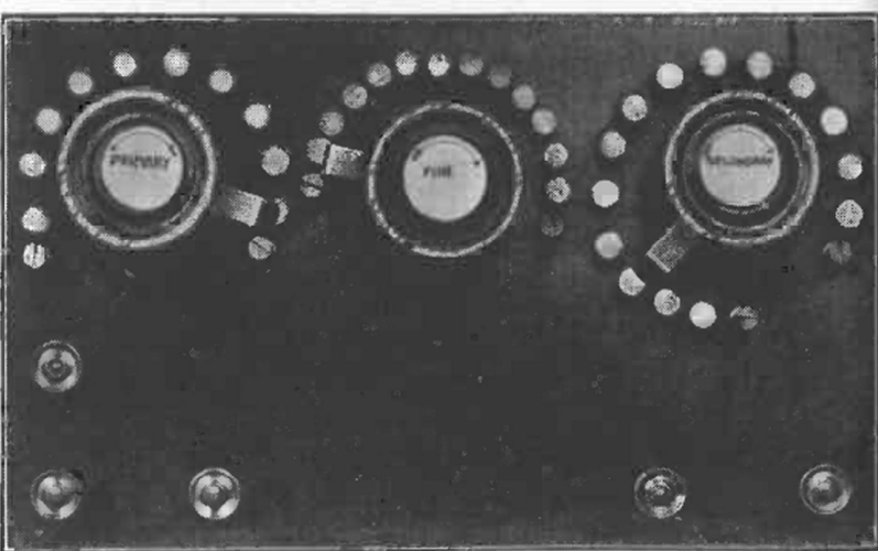
Fig. 34.—Photograph of Panel and Tuning Switches.
