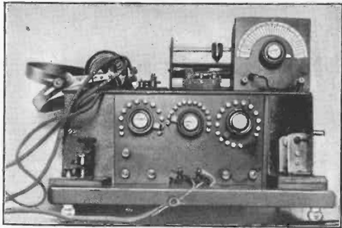
Fig. 3.—The Receiving Set in Complete Detail.
