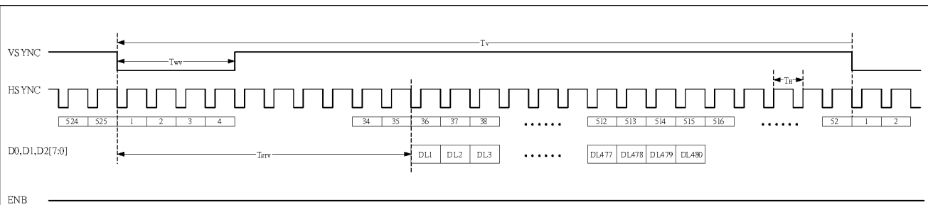
VERTICAL TIMING
