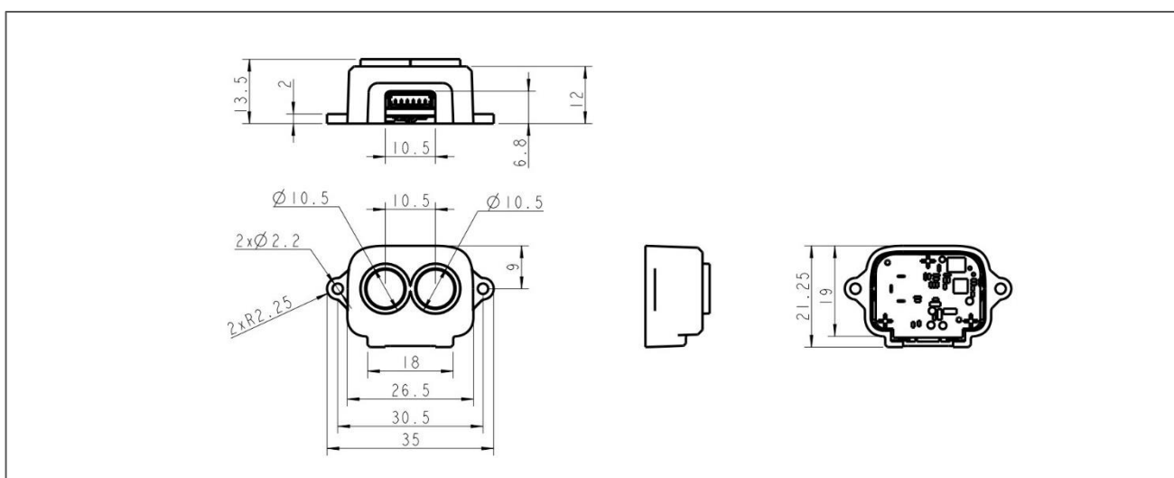
Figure 1 TF-Luna dimensions (Unit: mm)
