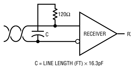
Figure 10. AC Coupled Termination
