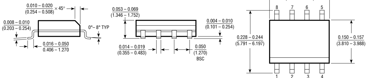
S8 Package 8-Lead Plastic SOIC
