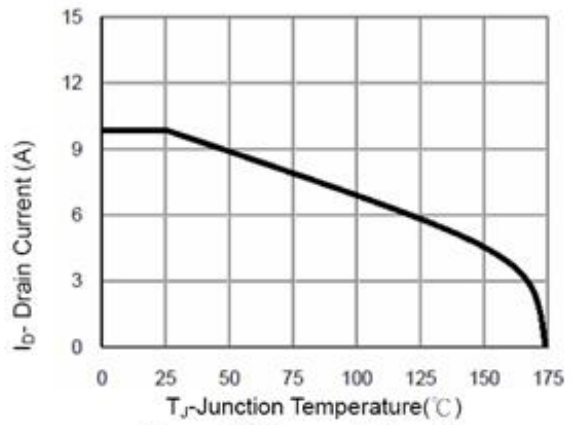
Figure 10 Current De-rating
