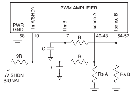
FIGURE 2. CURRENT LIMIT WITH OPTIONAL SHUTDOWN
