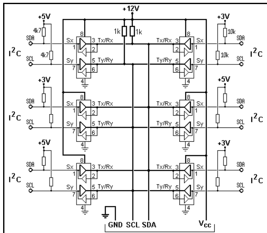
Figure 29. Distribute I 2 C using USB cables (1)
