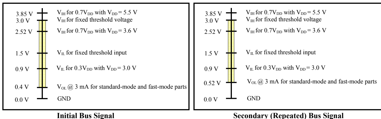
Figure 7. Voltage Level Comparison
