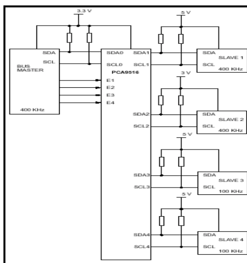
Figure 19. Typical Multiplexing Application
