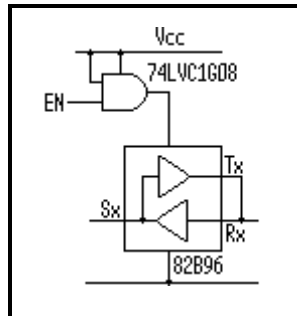
Figure 1. P82B96 Enable Input Configuration
