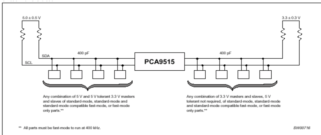
Figure 18. Typical Voltage Translation Application
