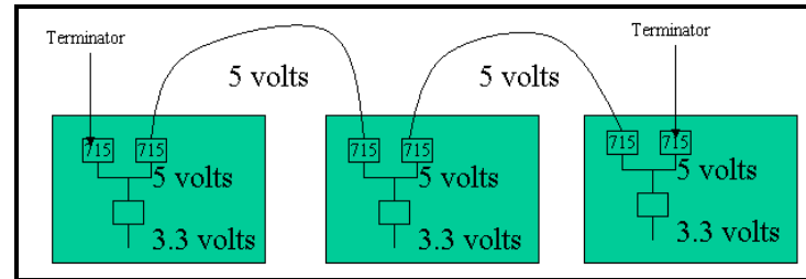
Figure 35. Multi-drop application using P82B715
