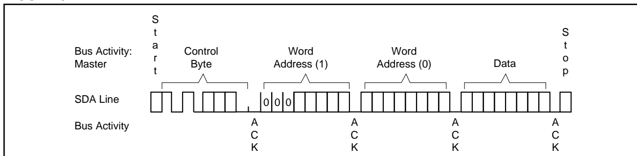
FIGURE 5-1: BYTE WRITE
