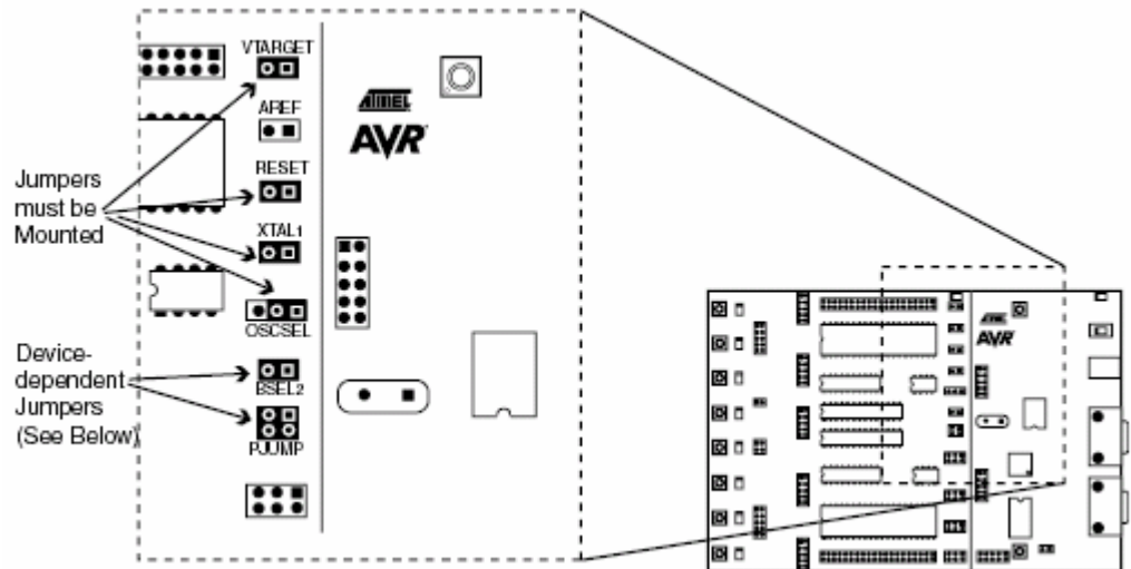
Abbildung 3. 19: Jumper Settings zur High-voltage Prog.
