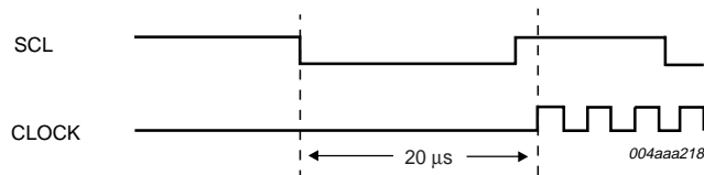
Fig 8. Clock wake up using SCL.
