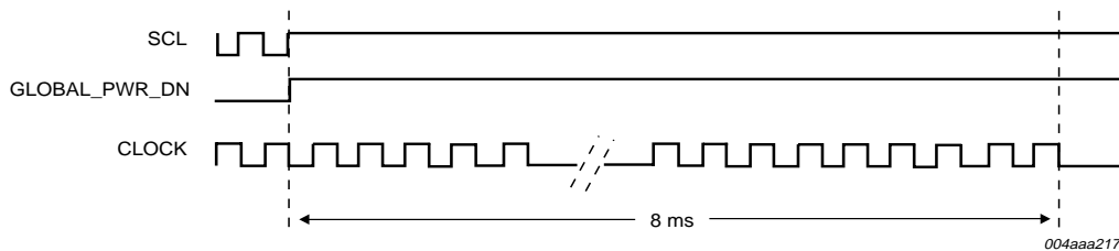
Fig 7. Clock stopped using the GLOBAL_PWR_DN bit.
