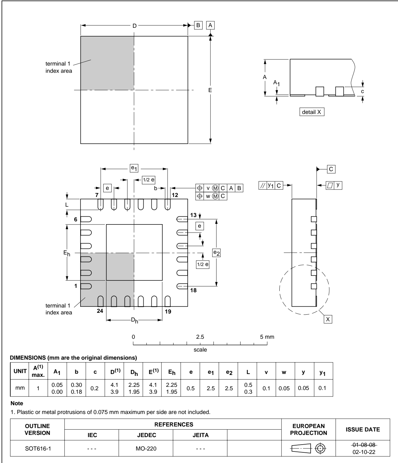
Fig 27. HVQFN24 package outline.
