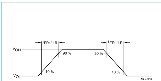
Fig 16. Rise and fall times.
