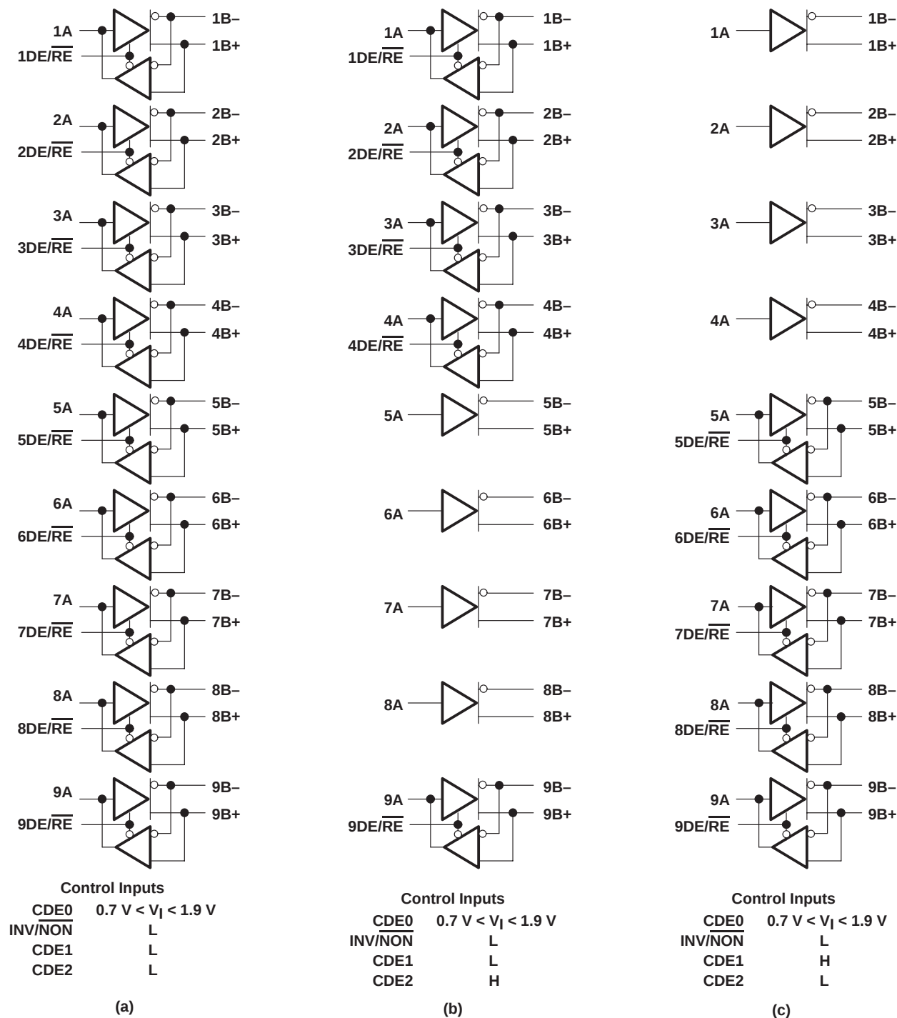
Figure 9. Logic Diagrams
