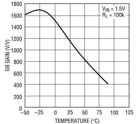
"Gain Block" Gain
