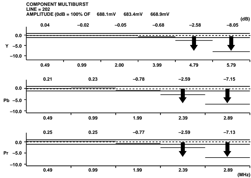
Figure 90. PAL YUV Multiburst Response
