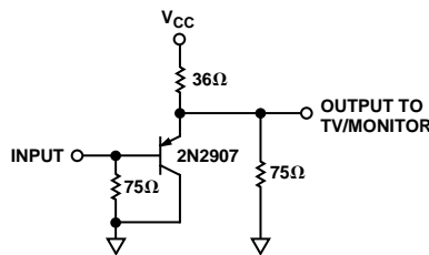
Figure 72. Recommended Output DAC Buffer
