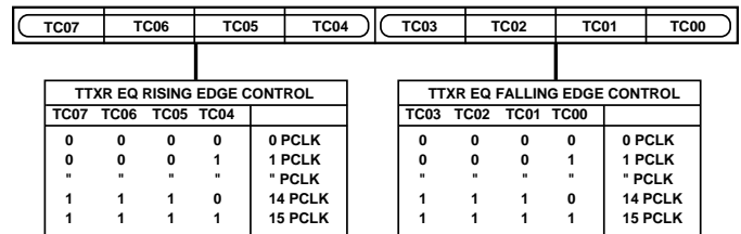
Figure 43. Teletext Control Register
