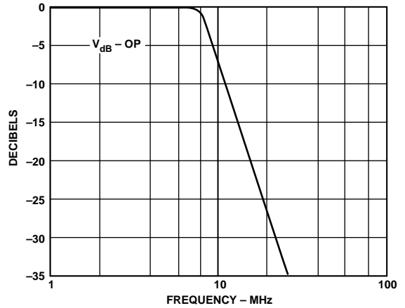
Figure 69. Output Filter Close Up
