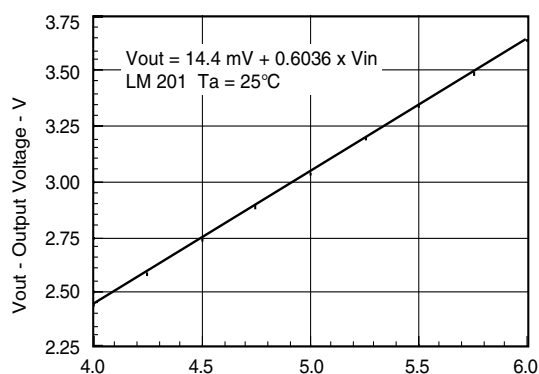
Figure 19. Transfer Gain
