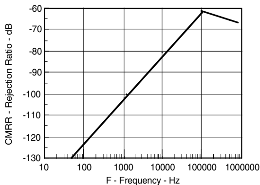
Figure 14. Common-Mode Rejection
