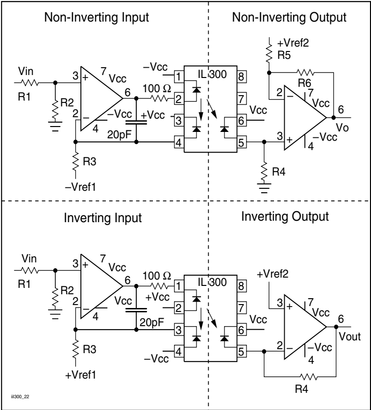
Figure 22. Non-inverting and Inverting Amplifiers
