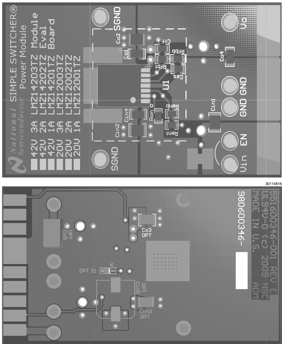
FIGURE 1. Top and bottom view of evaluation PCB
