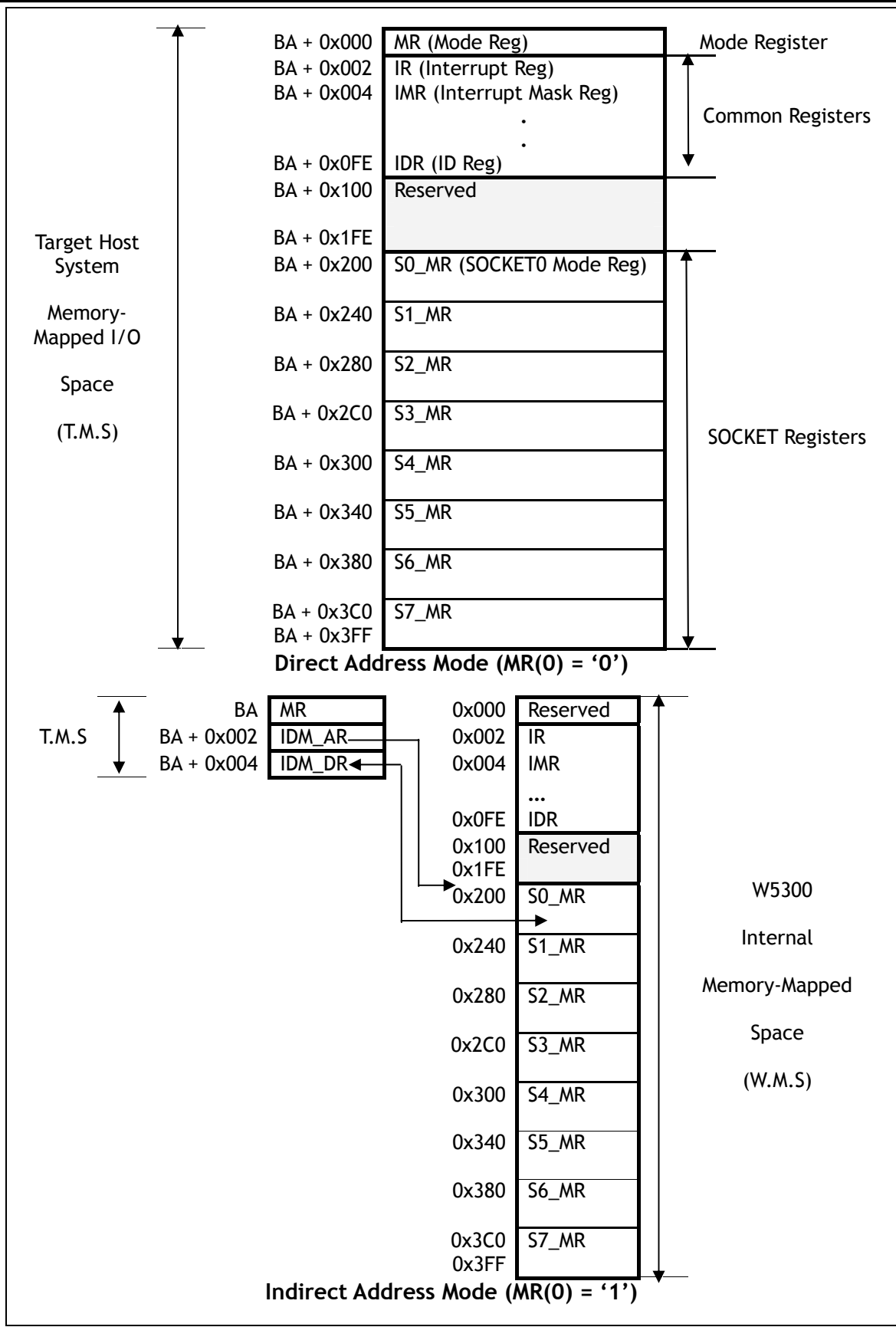
Fig 3. Memory Map
