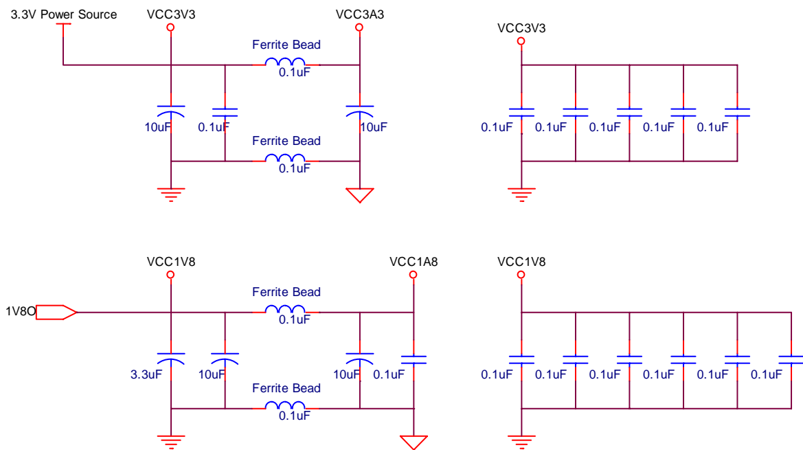
Fig 2. Power Design
