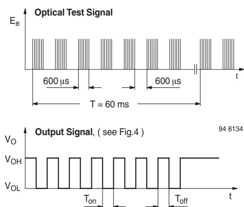
Figure 3. Output Function
