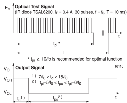
Figure 1. Output Function
