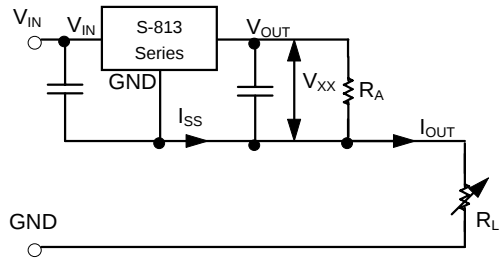
Figure 25 Constant current regulator
