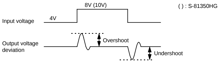
Type II : Square wave from 0V to 10V
