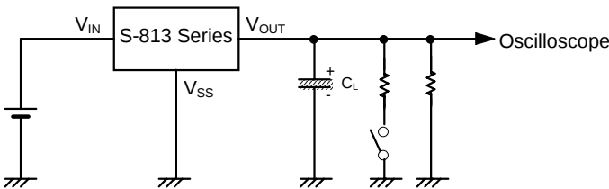
Figure 13 Measuring circuit
