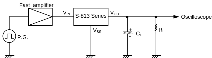
Figure 9 Measuring circuit
