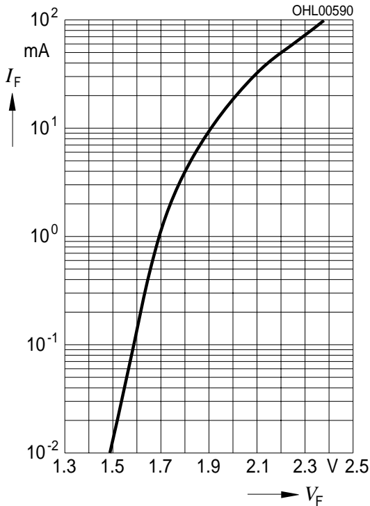
Durchlassstrom I_F = f(V_F) Forward Current T_A = 25\text{ °C}
