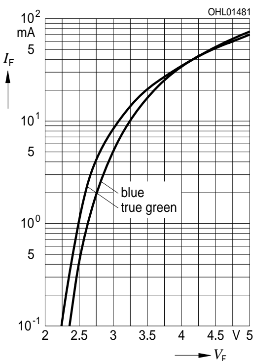
Durchlassstrom I_F = f(V_F) Forward Current T_A = 25\text{ °C}
