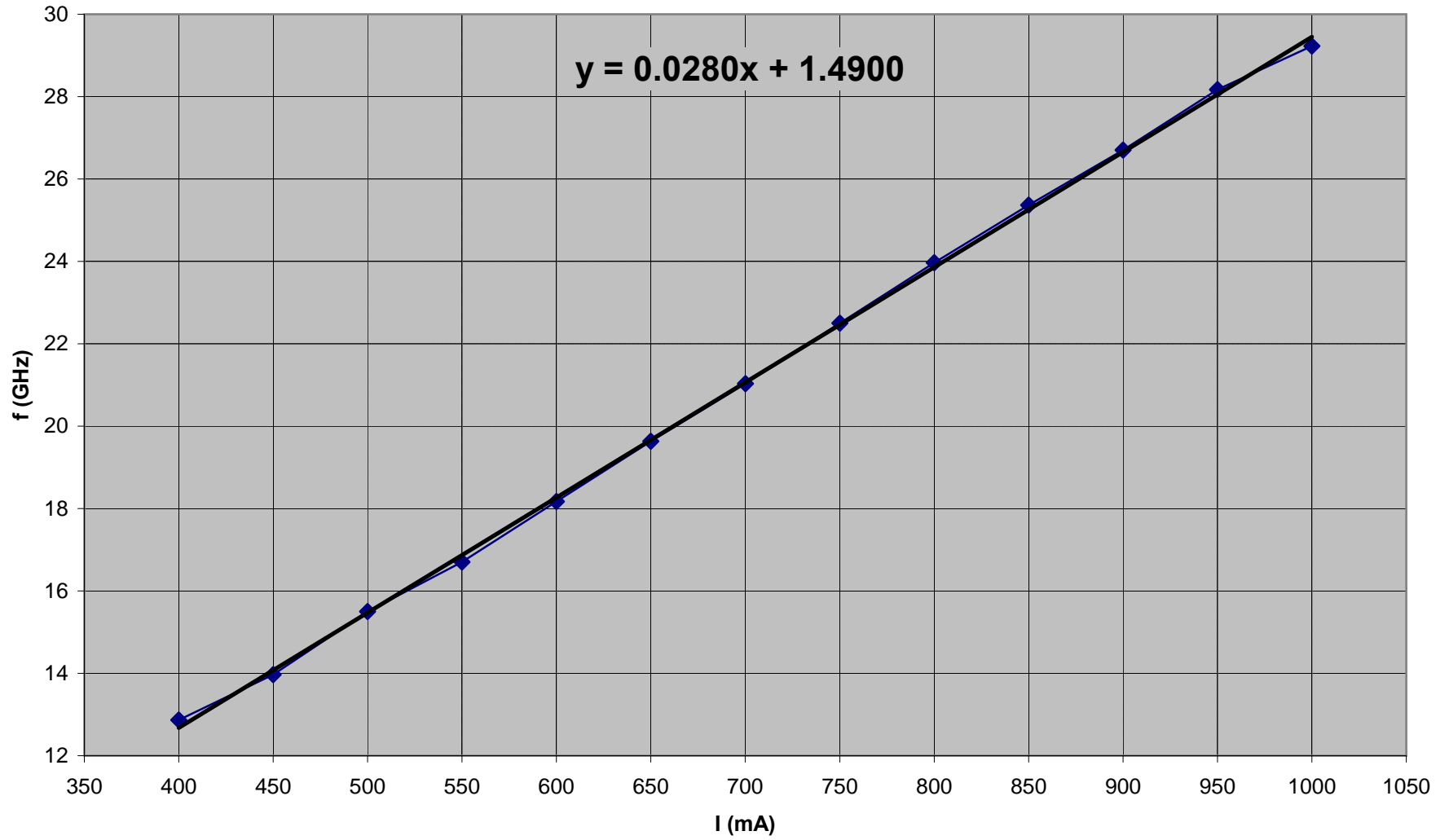
Wiltron YIG (heater not connected) current source: HP E3615A (0-20V, 0-3A)
