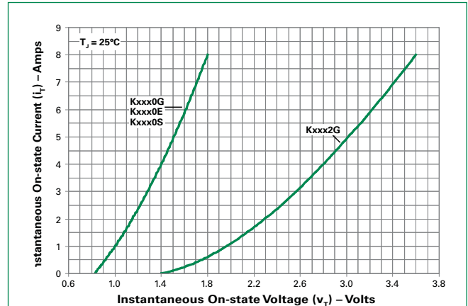
Figure 2: On-state Current vs. On-state Voltage (Typical)
