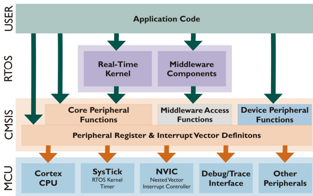
Figure 2 CMSIS Structure functional flow
