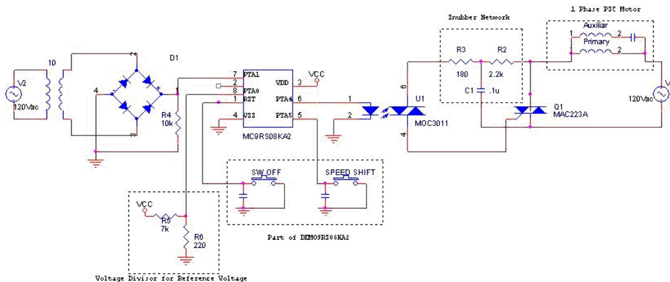
Figure 13. Complete Circuit
