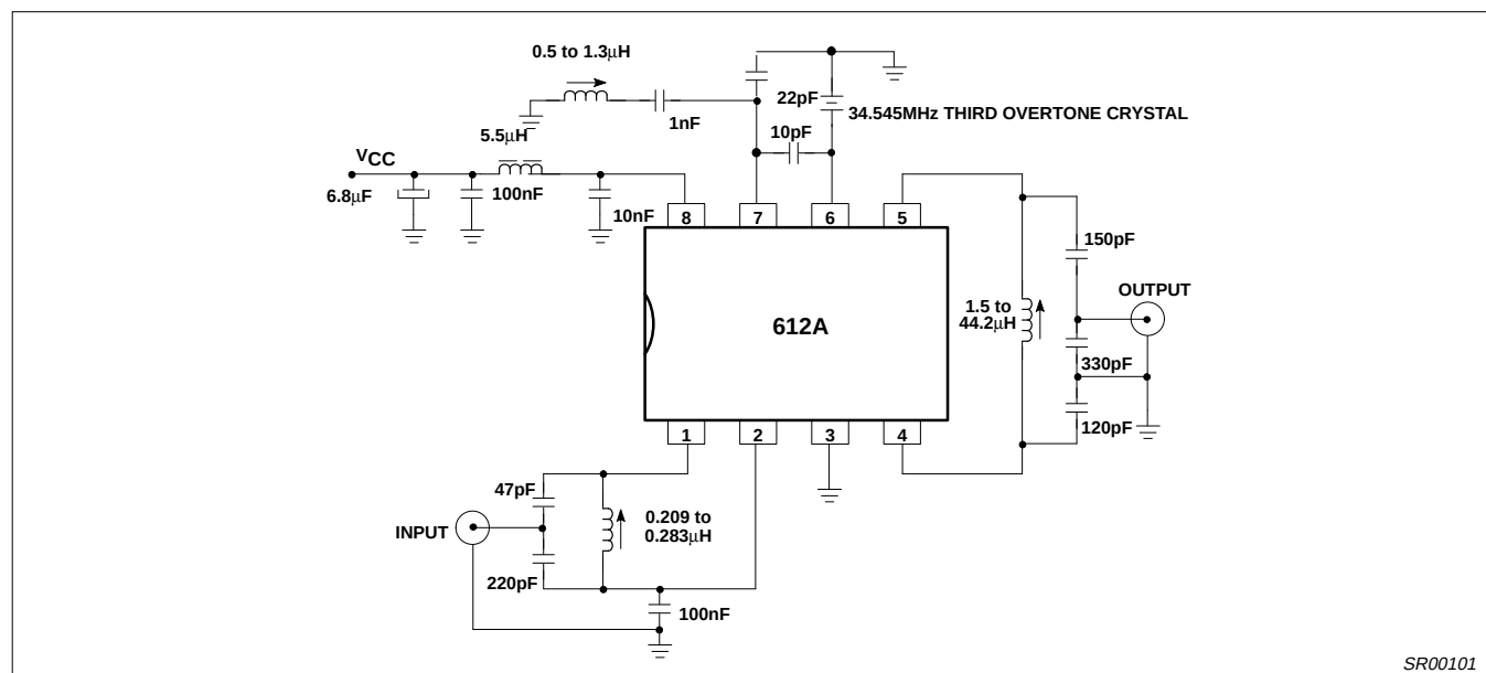
Figure 3. Test Configuration
