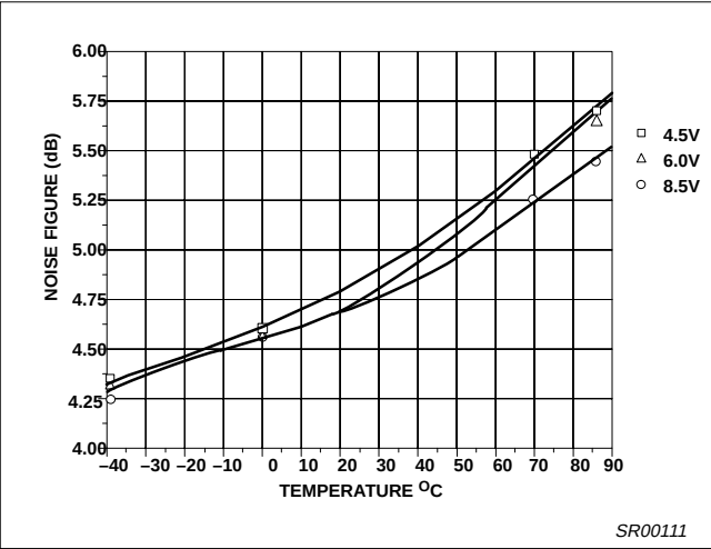
Figure 13. Noise Figure
