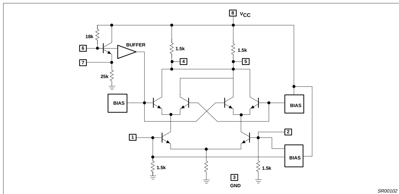
Figure 4. Equivalent Circuit
