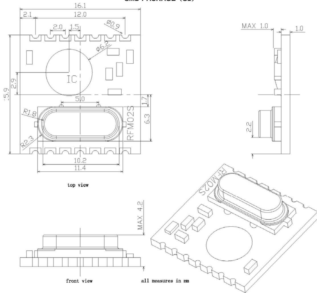
SMD PACKAGE (S2)
