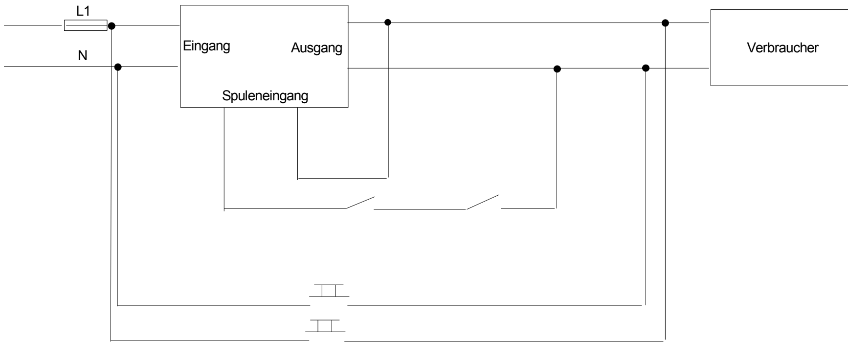
Schlüsseltaster 2-Polig
