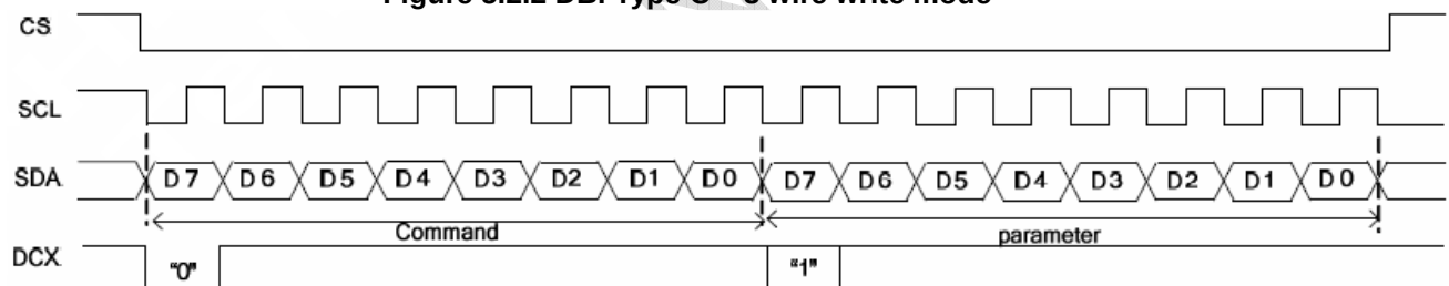
Figure 5.2.3 DBI Type C – 4wire write mode
