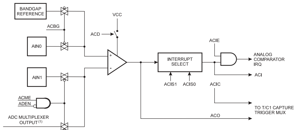
Figure 100. Analog Comparator Block Diagram (2)
