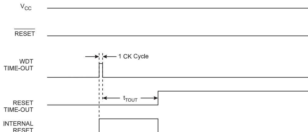
Figure 21. Watchdog System Reset During Operation
