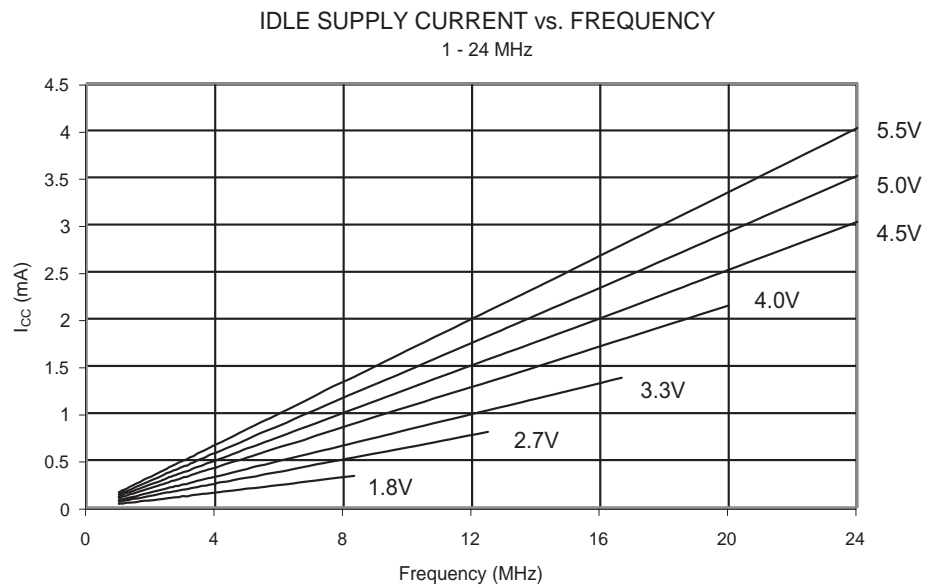
Figure 143. Idle Supply Current vs. Frequency (1 - 24 MHz)
