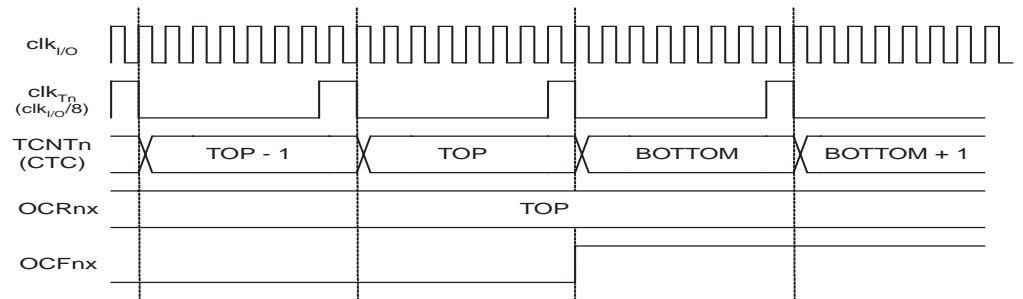
Figure 64. Timer/Counter Timing Diagram, Clear Timer on Compare Match mode, with Prescaler ( f_{clk\_I/O}/8 )
