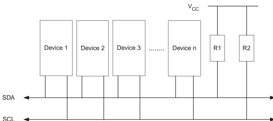
Figure 78. TWI Bus Interconnection
