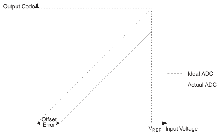
Figure 110. Offset Error
