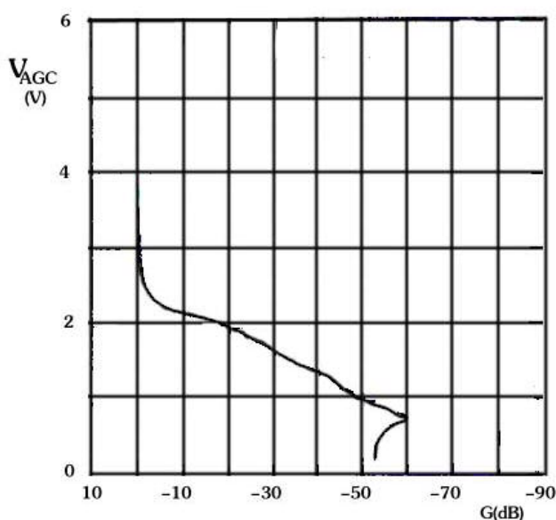
AGC characteristics Channel S8
